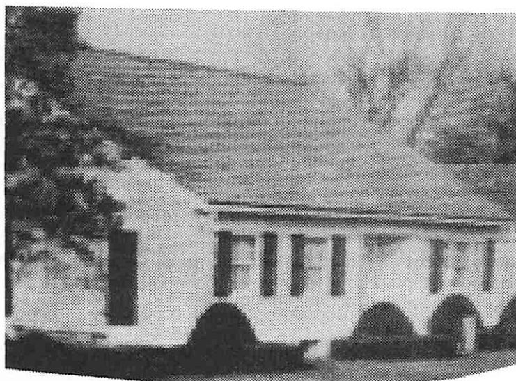
(c) Blue
