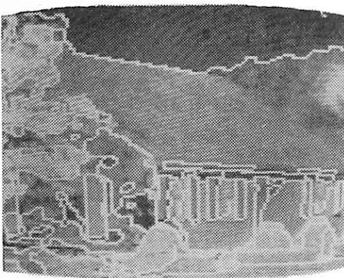
\bar{R}
