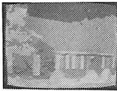
iteration 5
