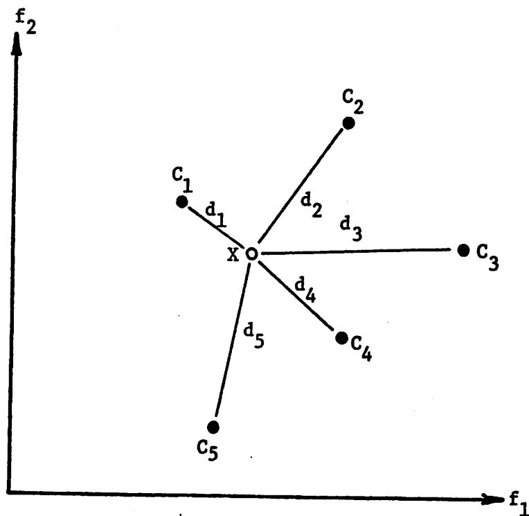
Figure 9. Initial Probabilities of Cluster Labels. The initial probability that histogram point X belongs to cluster C_1 will be a function of distance d_1 relative to the set of d_j, j \neq 1 .
