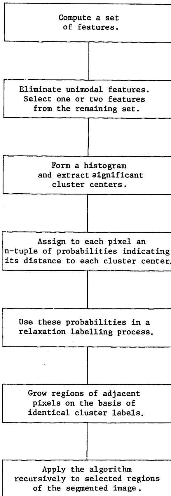
Figure 3. Segmentation Algorithm Overview.
