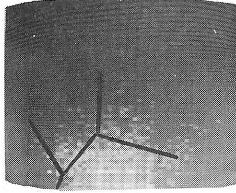
(e) Cluster 5
