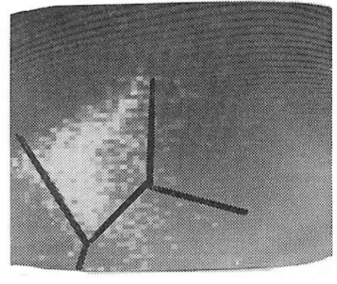
(f) Cluster 6
