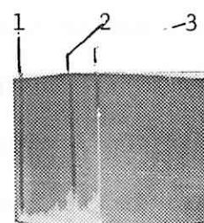
(c) Blue
