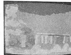
iteration 25
