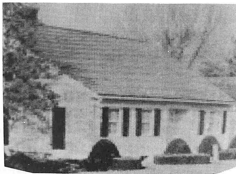
(b) Green
