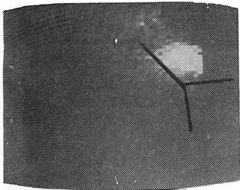
(a) Cluster 1
