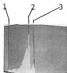
(a) Red
