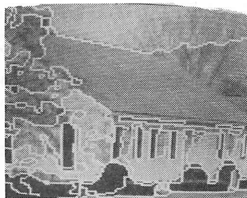
intensity
