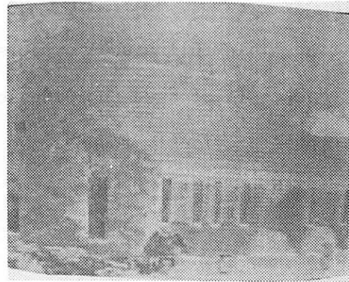
(b) \bar{G}
