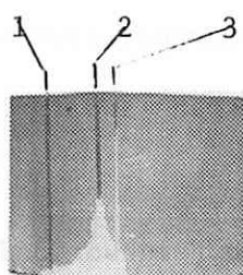
(b) Green
