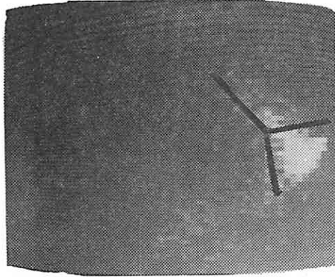
(b) Cluster 2
