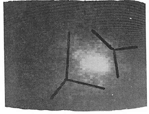
(c) Cluster 3
