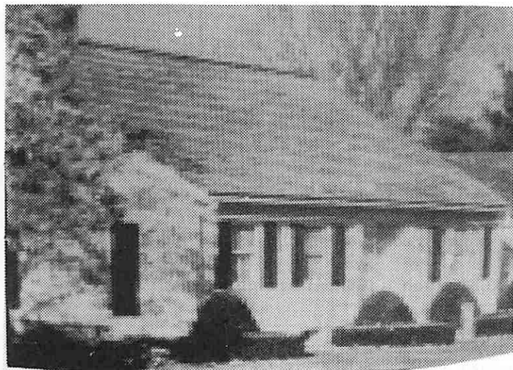
(a) Red
