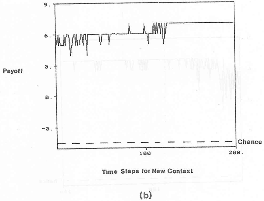
Figure 8. Example 3. With the associative matrix obtained after training in Example 2, context vector X1 of Fig. 7a was corrupted by additive noise and presented to the ASN. E implemented payoff function Z1. a) The corrupted context vector, the optimal output pattern, and the ASN's initial guess. b) ASN payoff as it searches for the optimal output pattern.
