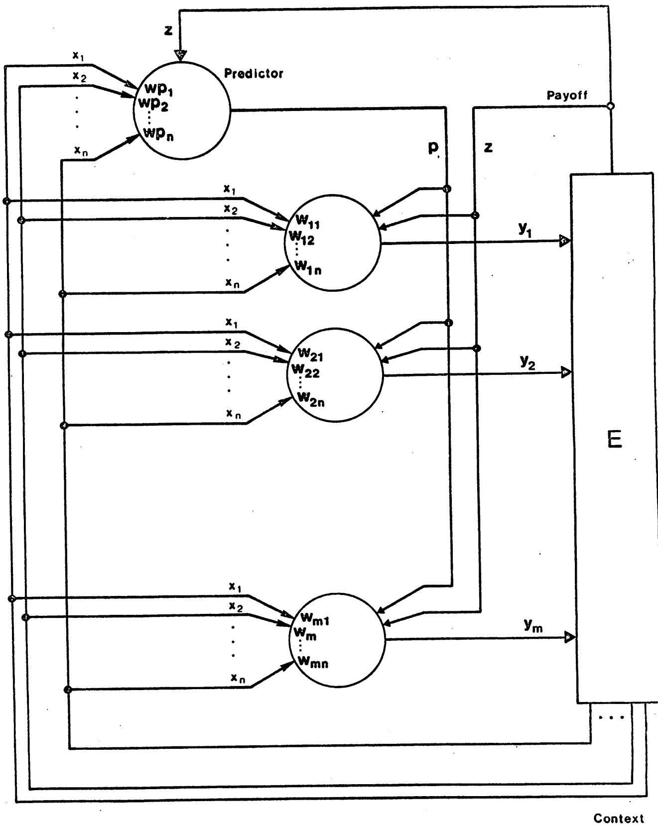
Figure 3. An ASN consisting of m adaptive elements and one predictor. The adaptive element weights form an m \times n associative matrix.
