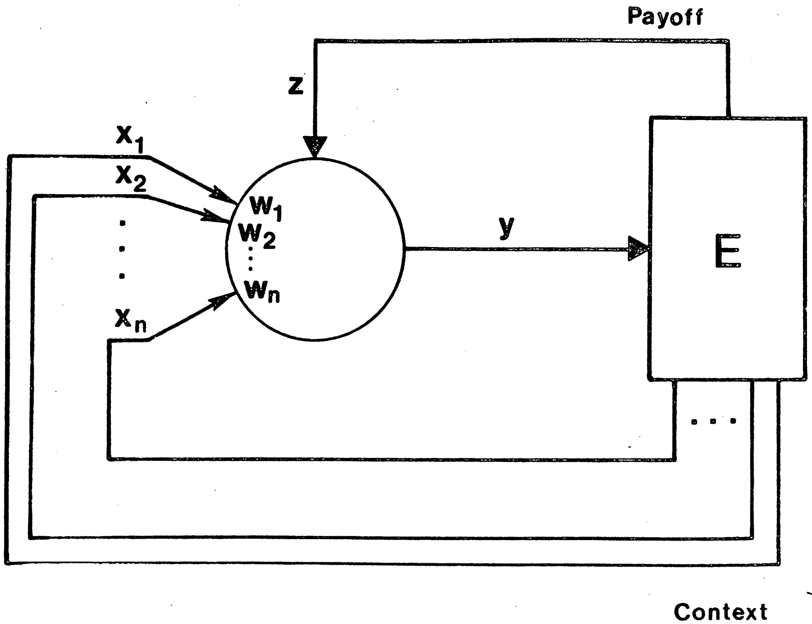
Figure 2. The simplest ASN: A single adaptive element interacting with an environment E.
