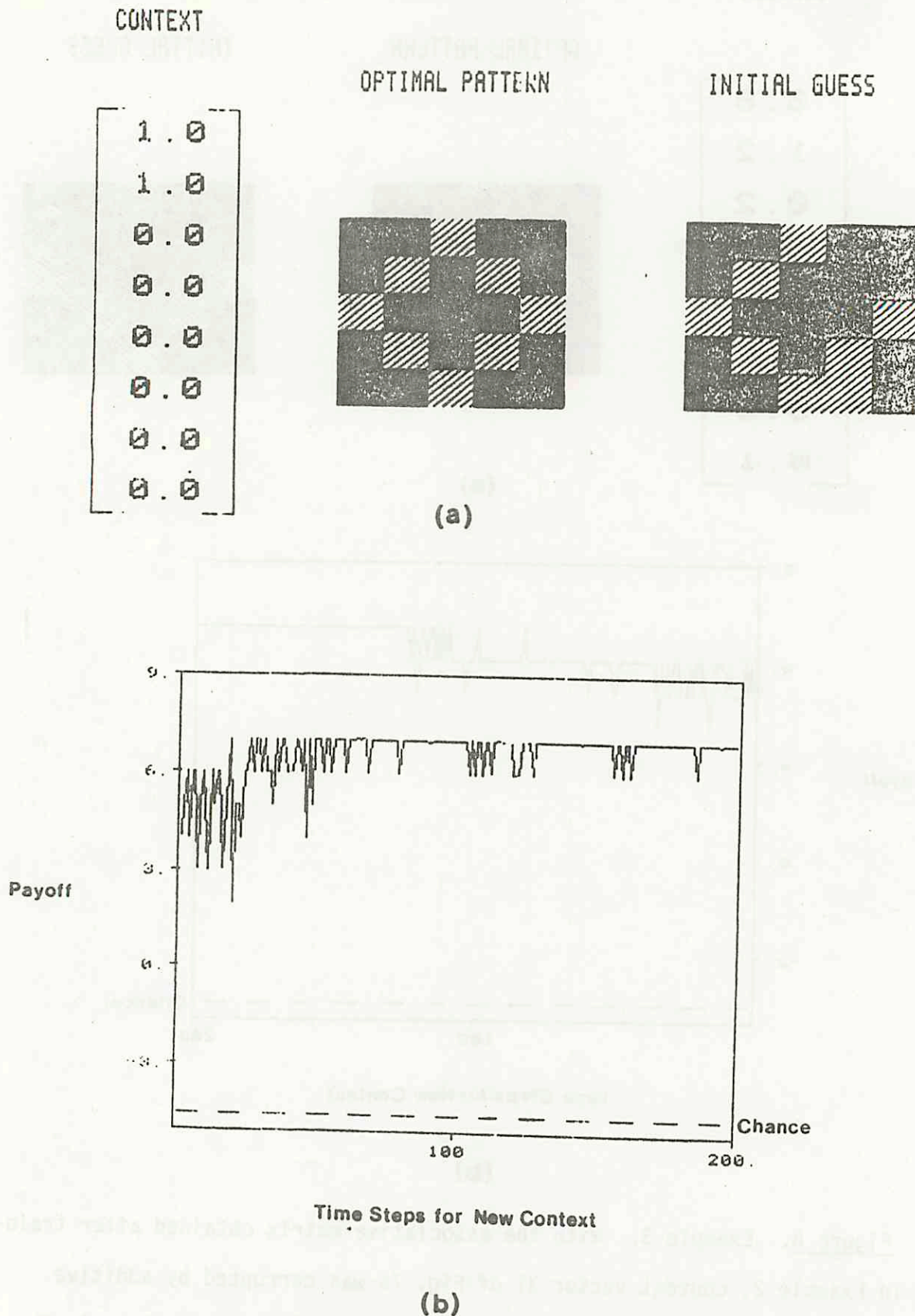
Figure 9. Example 4. With the associative matrix obtained after training in Example 2, a fragment of X_1 was presented as context. Implemented payoff function Z_1 . a) The fragment of X_1 , the optimal pattern, and the initial guess. b) ASN payoff as the search continues.
