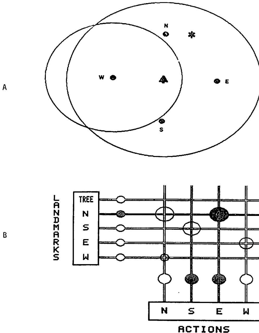
Figure 9. a) A spatial environment in which the attracting "tree" is surrounded by four other landmarks. The landmarks each possess a distinctive "odor" which can be sensed at a distance but which is not an attractant. Odor distributions decrease linearly from their associated landmarks and become undetectable at a certain distance (indicated for landmark 'W' by the surrounding circle). b) A network of goal-seeking adaptive elements. The five input pathways are labeled vertically on the left according to the landmarks to which they respond. The shaded input pathway N indicates that the organism is near the north neutral landmark. The four output pathways controlling actions are labeled horizontally at the bottom according to the direction of movement they cause. The shaded output elements indicate that a southeast movement is being made. The associative matrix weights are displayed as circles centered on the intersections of the horizontal input pathways and vertical output pathways. Positive weights are shown as hollow circles, and negative weights are shown as solid circles. (Reprinted from Barto and Sutton, 1981a).
