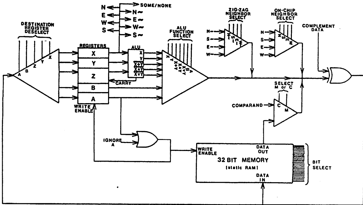
Organization of One PE
