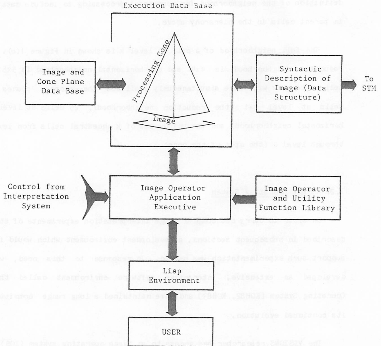
Figure 2. Block Diagram of the Image Operating System.
