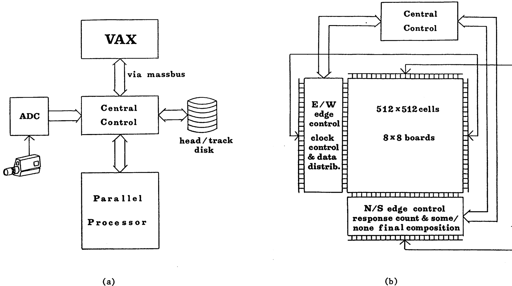
Figure 19. Organization of CAAPP.
