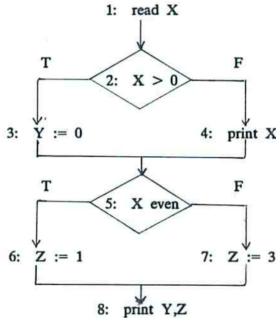
Figure 10: Data Flow Testing Example.
