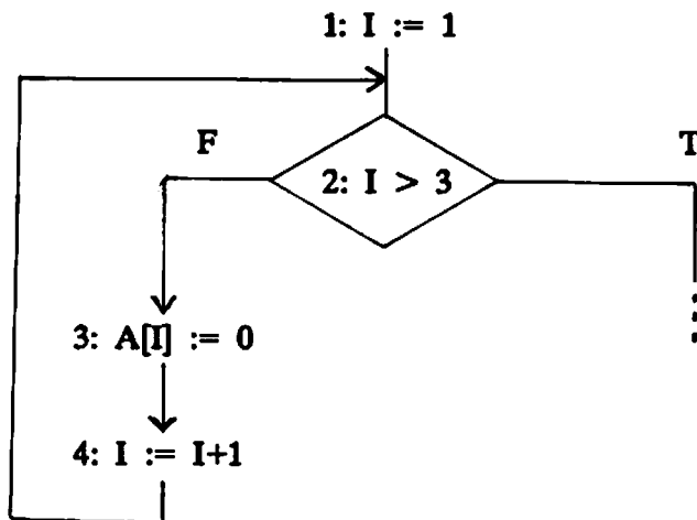
Figure 8: Array Element Determination.
