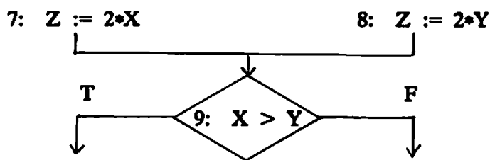
Figure 11: Perturbation Testing Example.
