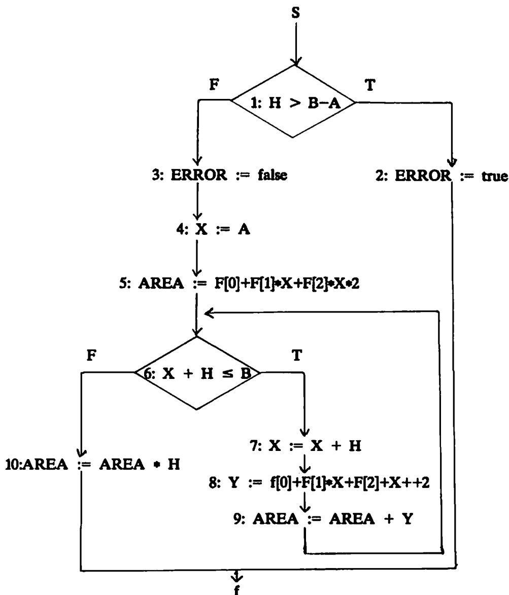
Figure 2: Control Flow Graph for RECTANGLE.
