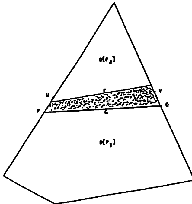
Figure 12: Domain Testing Strategy.
