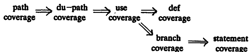
Figure 9: Data Flow Testing Criteria.
