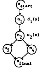
Figure 7: Module M_6 and its control flow graph G(M_6) .
