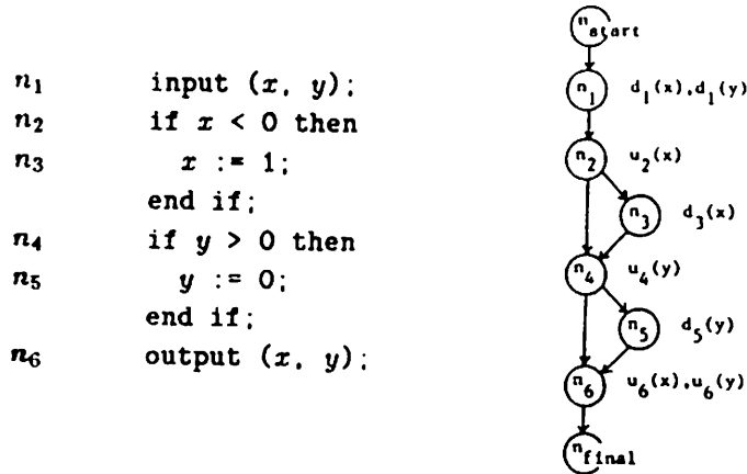
Figure 3: Module M_2 and its control flow graph G(M_2) .
