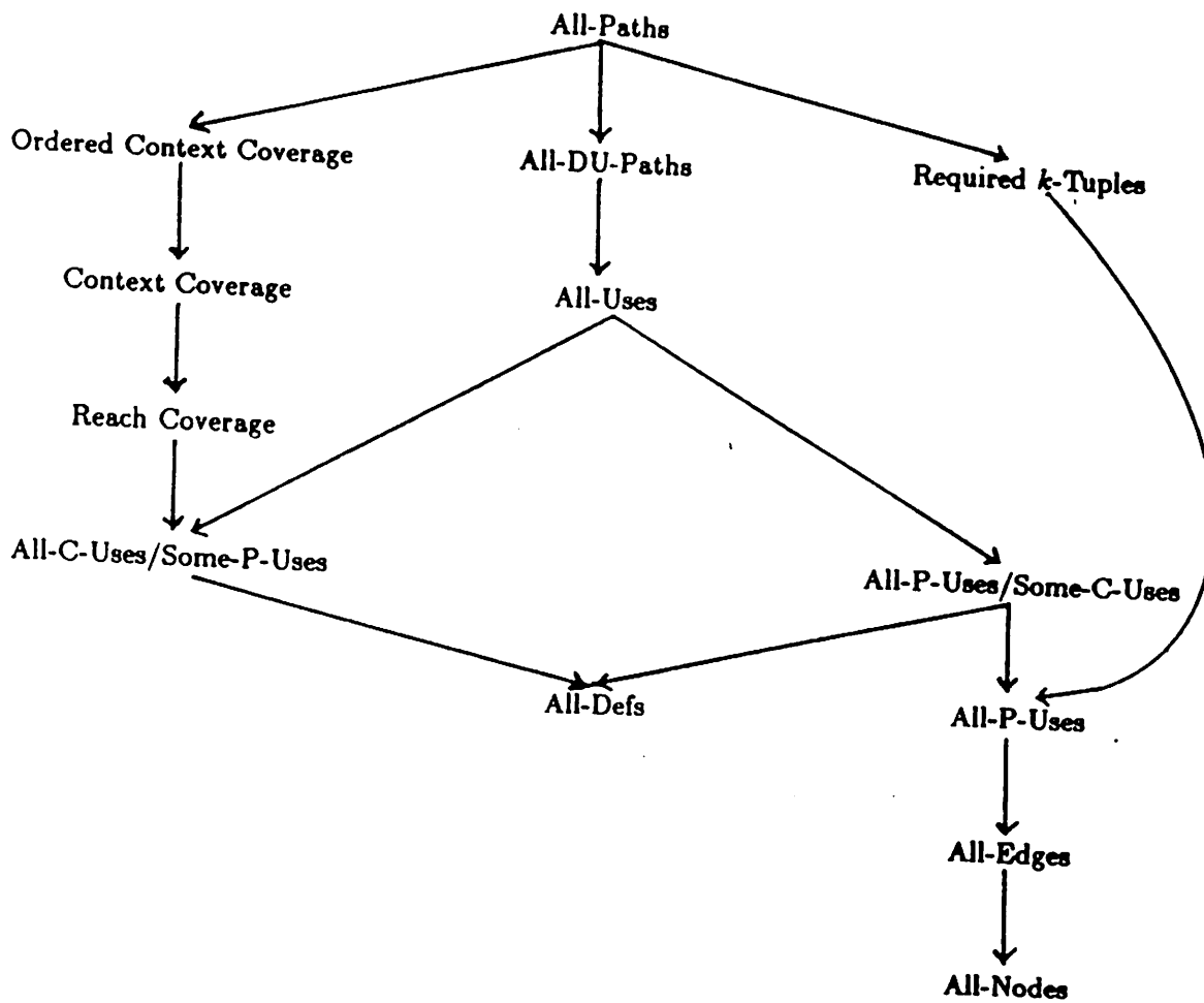
Figure 9: The New Subsumption Hierarchy.
