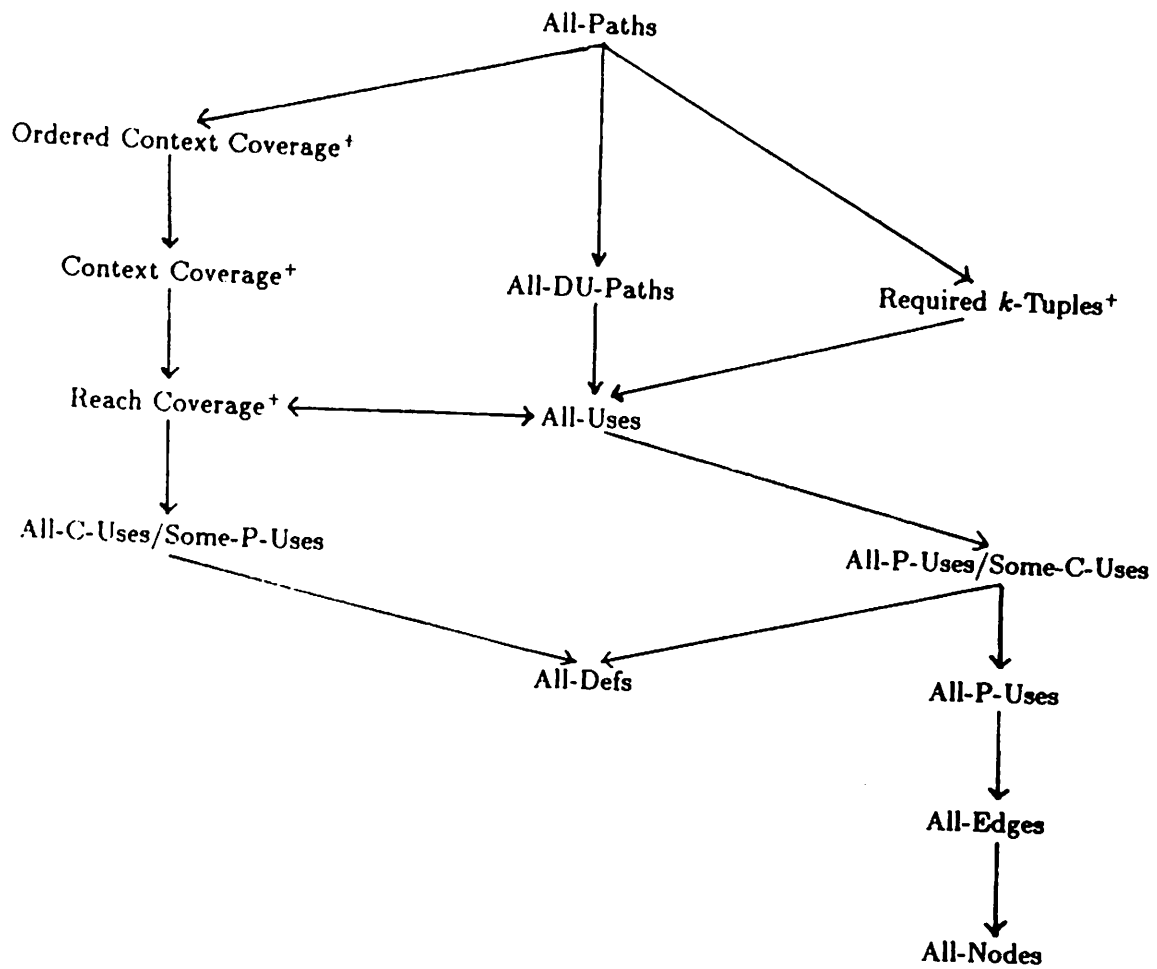
Figure 10: The Final Subsumption Hierarchy.
