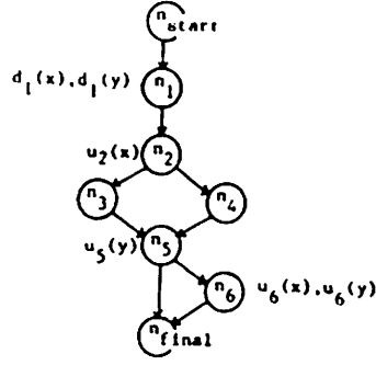
Figure 10: Module M_9 and its control flow graph G(M_9) .
