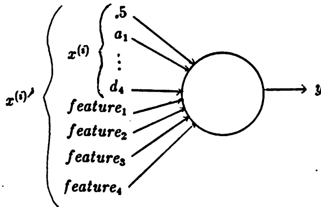
Figure 9: Multiplexer Task—Original Representation Plus New Features
