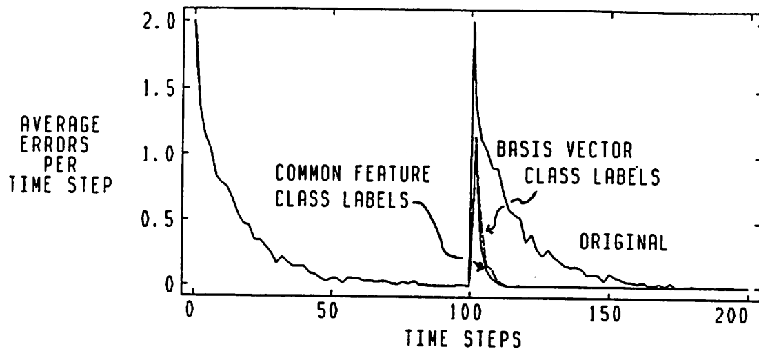
Figure 14: Input-Cluster Task—Learning Curves
