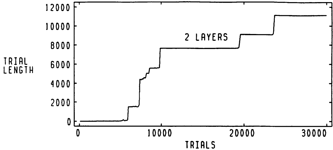
Figure 34: Balancing Time versus Trials for Two-Layer System
