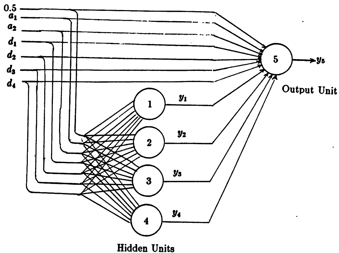
Figure 23: Two-Layer Network for Multiplexer Experiments
