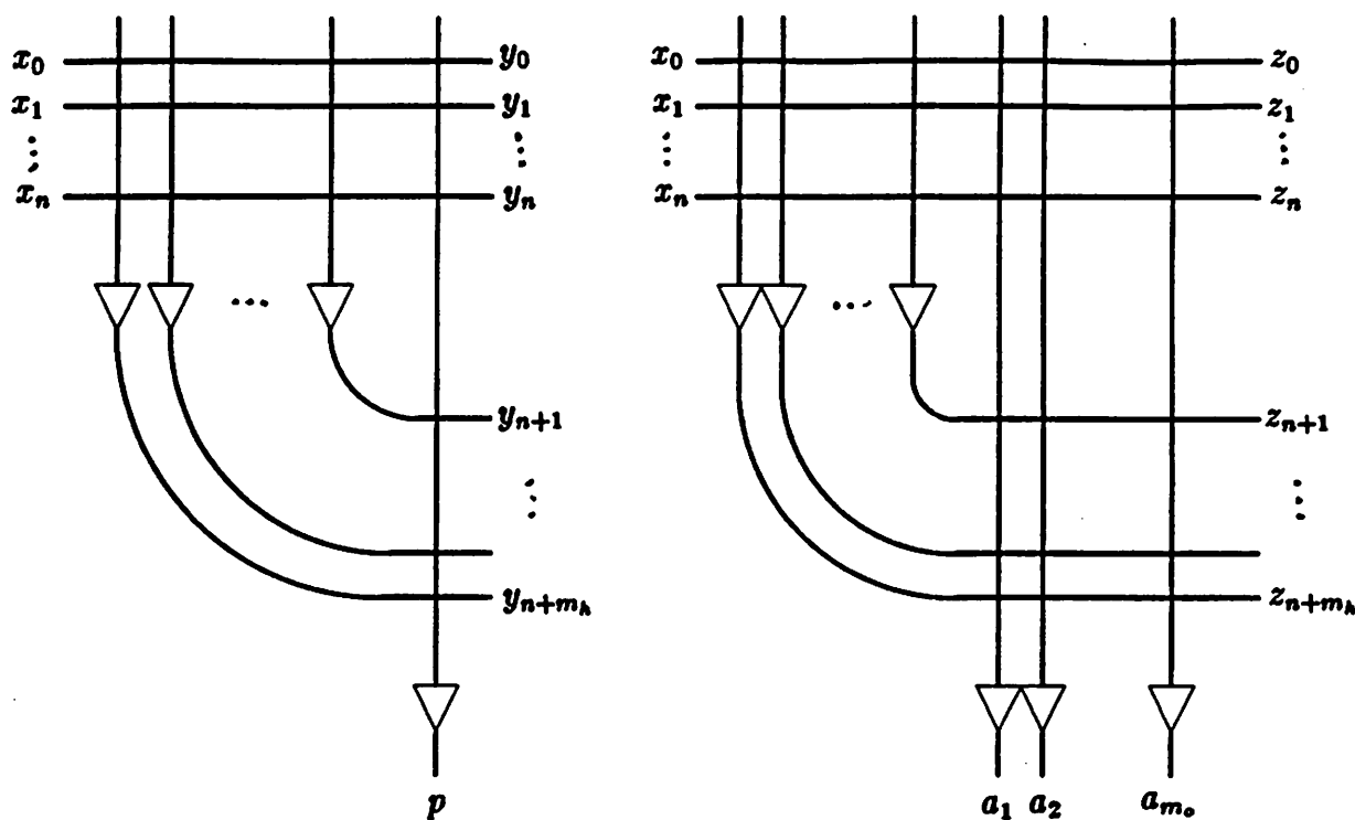
Figure 28: Two-Layer Networks for Strategy Learning
