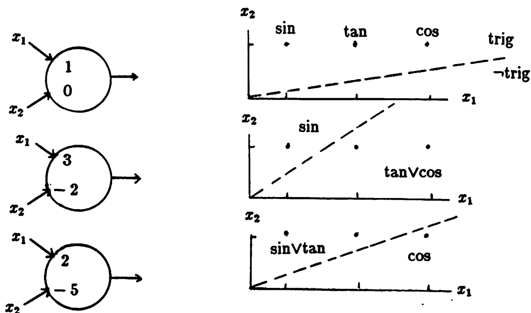
Figure 5: Possible Concepts using Connectionist Representation
