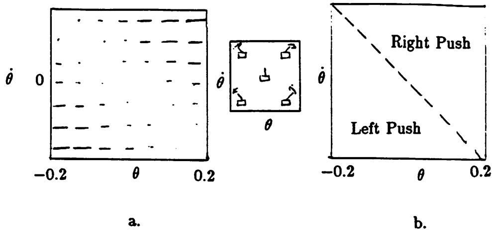
Figure 30: Desired Functions for Pole-Balancing Solution
