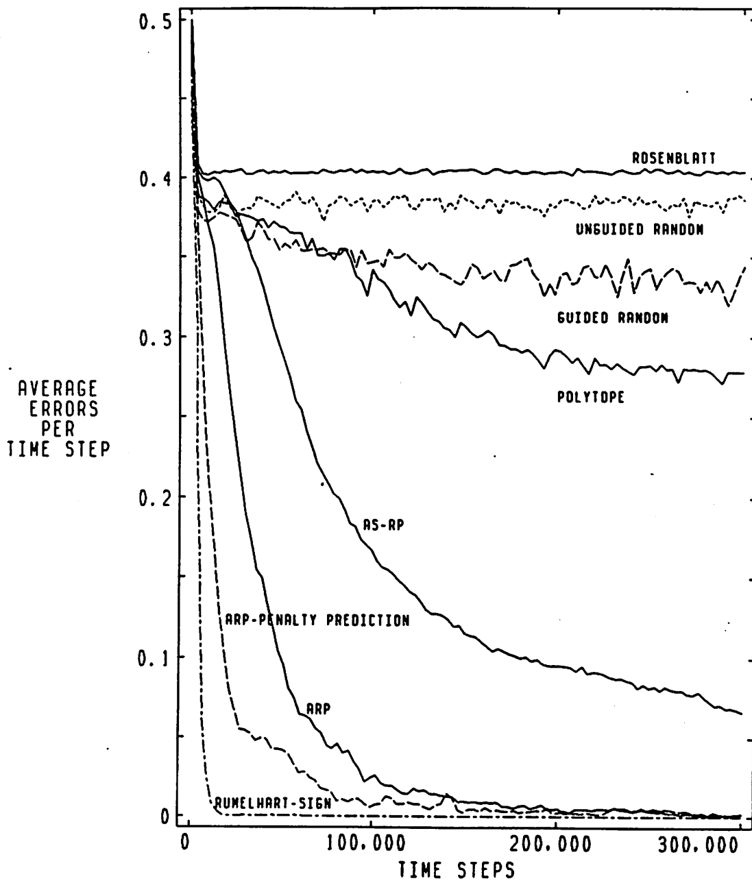
Figure 27: Learning Curves for All Algorithms on the Multiplexer Task
