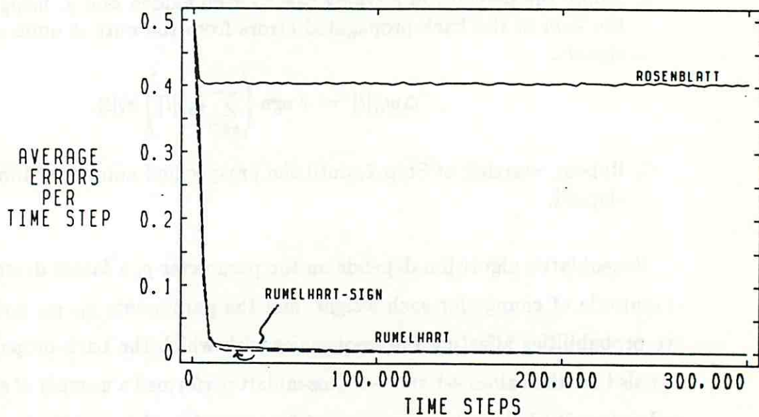
Figure 25: Learning Curve for Error-Correction Algorithms on the Multiplexer Task
