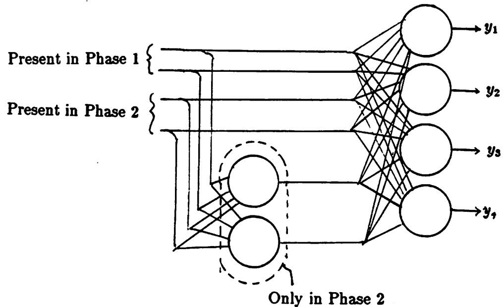
Figure 16: Output-Vector Task—Hidden Units That Correlate Output Units
