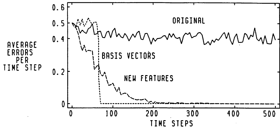
Figure 10: Multiplexer Task—Learning Curves
