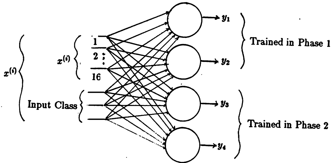
Figure 12: Input-Cluster Task—Basis Vectors as Class Labels
