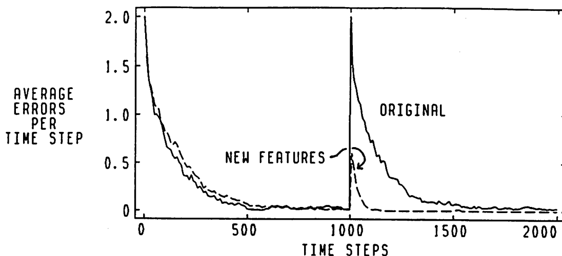
Figure 17: Learning Curves for the Output-Vector Task
