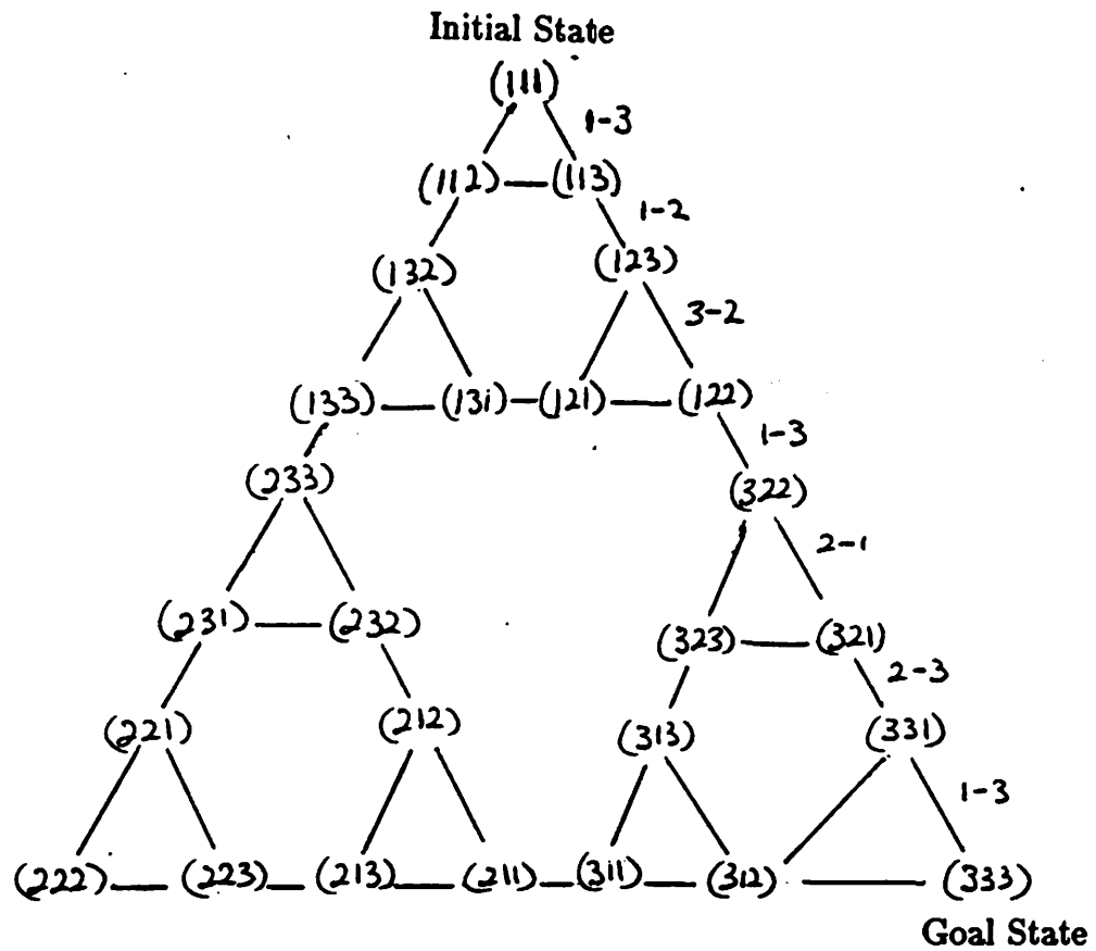
Figure 39: State Transition Graph for Three-Disk Tower of Hanoi Puzzle
