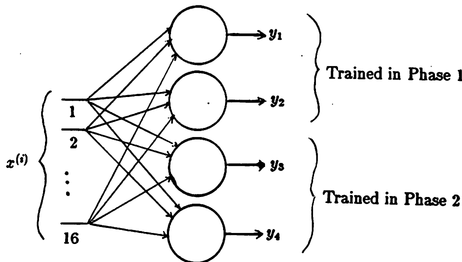
Figure 11: Input-Cluster Task—Original Representation
