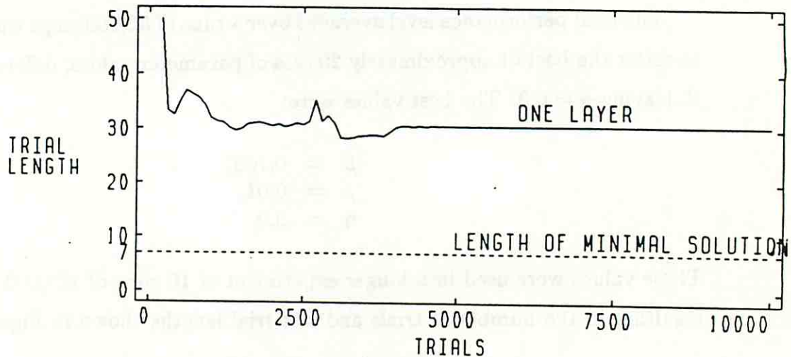
Figure 41: Length of Solution Path versus Trials for One-Layer System
