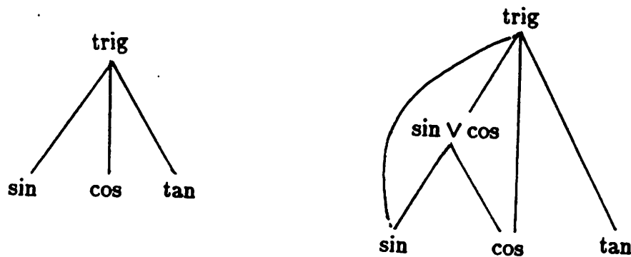
Figure 4: Adding a New Term to a Symbolic Representation
