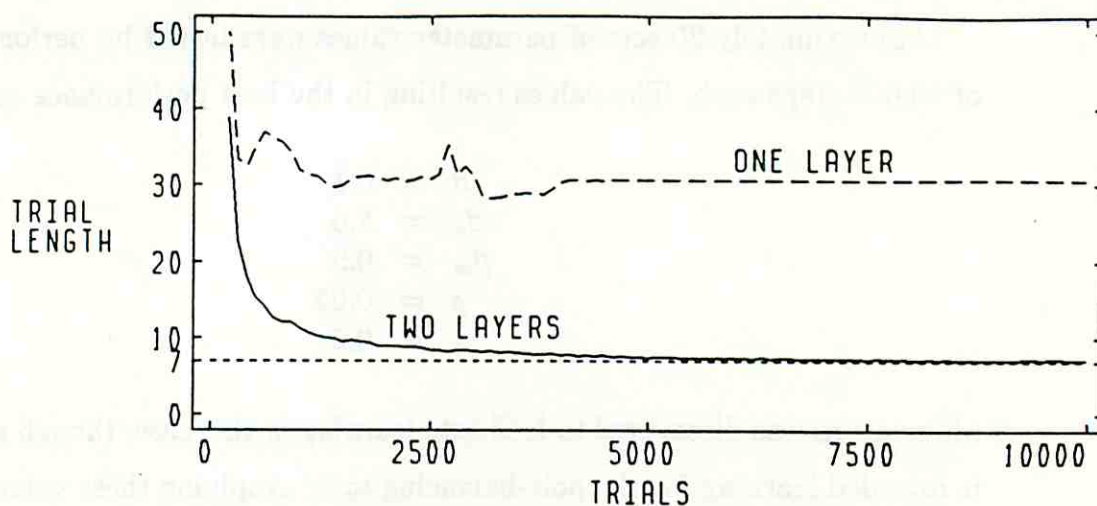
Figure 44: Length of Solution Path versus Trials for Two-Layer System
