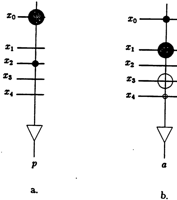
Figure 32: Weights Learned by One-Layer Network
