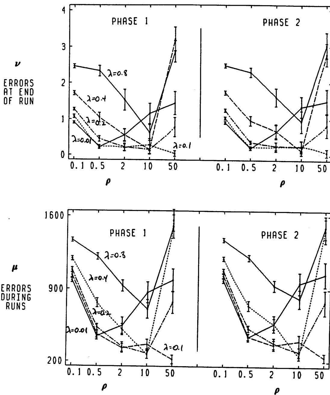
Figure 49: Output-Vector—Original Representation
