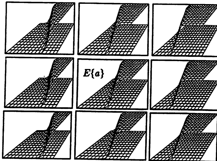
Figure 36: Functions Learned by Two-Layer Networks
