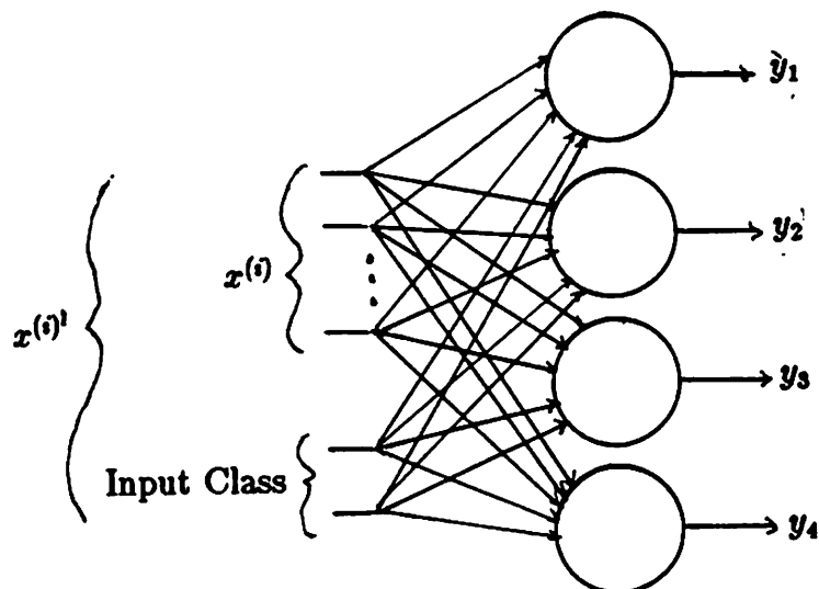
Figure 13: Input-Cluster Task—Class Labels with Common Feature
