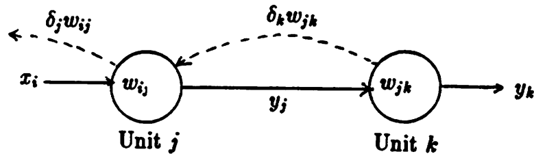
Figure 22: Back-Propagation of Gradient Information
