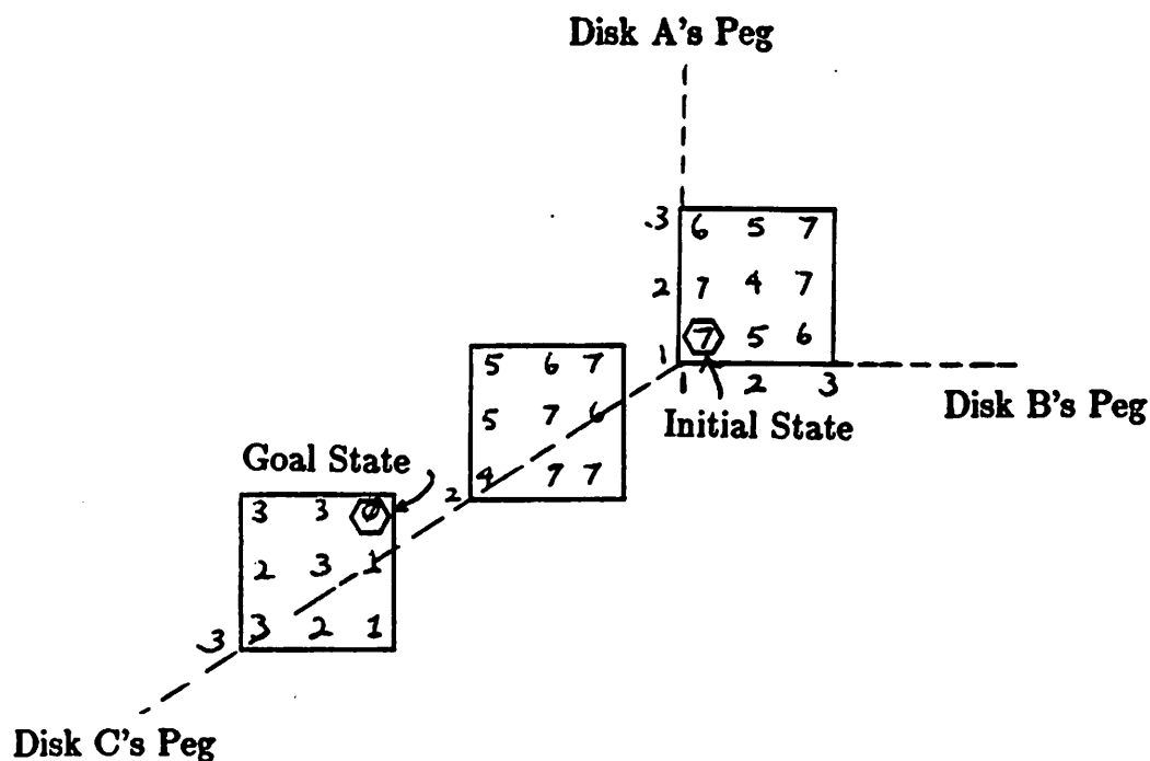
Figure 40: 3-Dimensional State Space and Desired Evaluations
