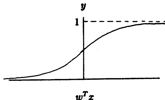
Figure 21: The Logistic Distribution
