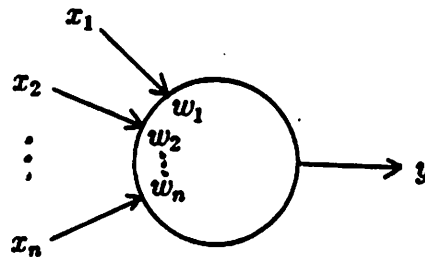
Figure 1: A Linear Threshold Unit
