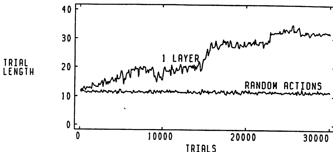
Figure 31: Balancing Time versus Trials for One-Layer System
