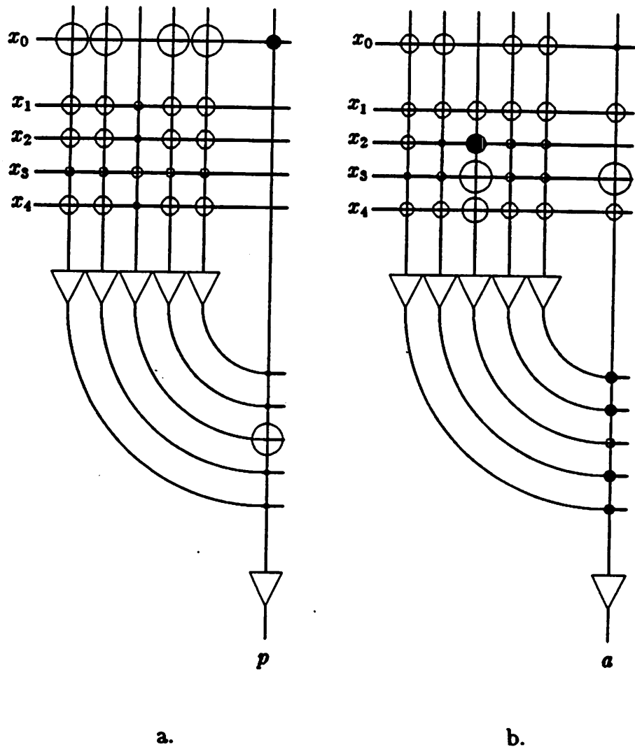
Figure 35: Weights Learned by Two-Layer Network
