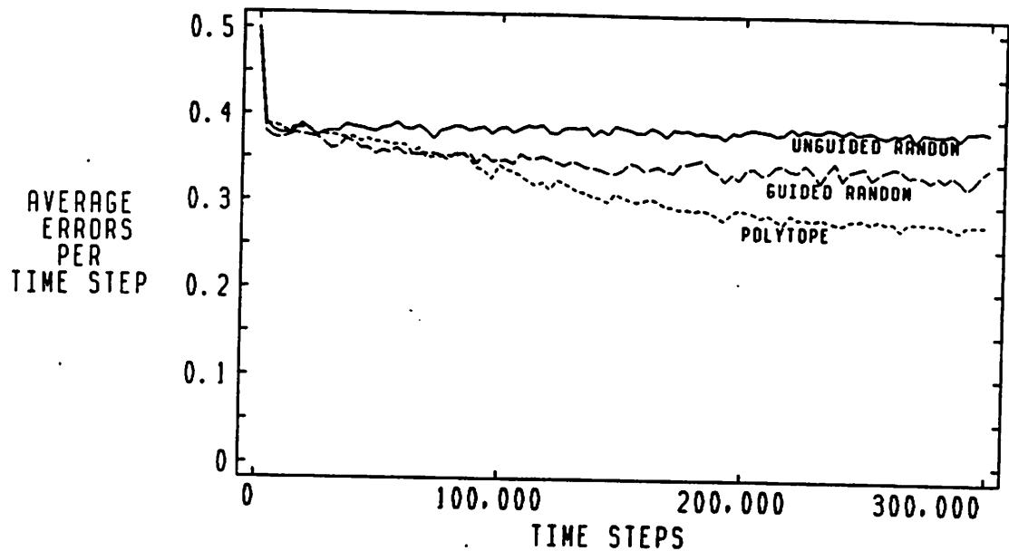
Figure 24: Learning Curves of Direct-Search Algorithms on the Multiplexer Task
