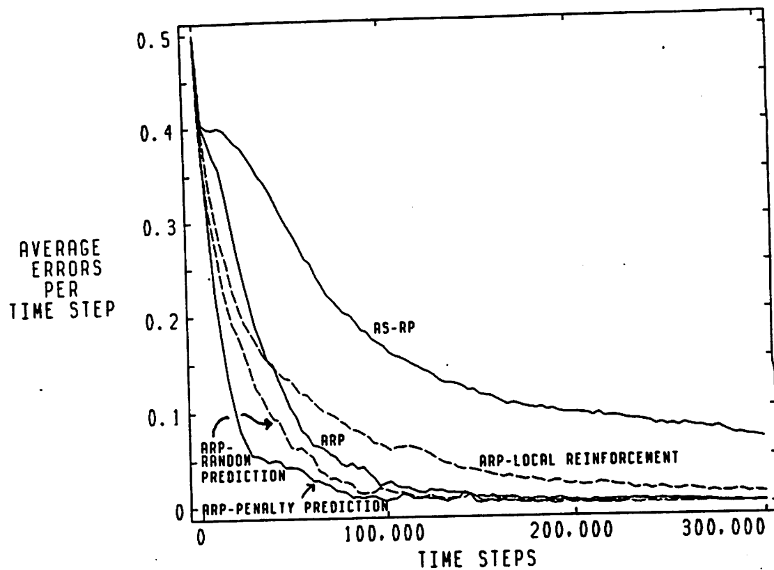
Figure 26: Learning Curve for Reinforcement Learning Algorithms on the Multiplexer Task
