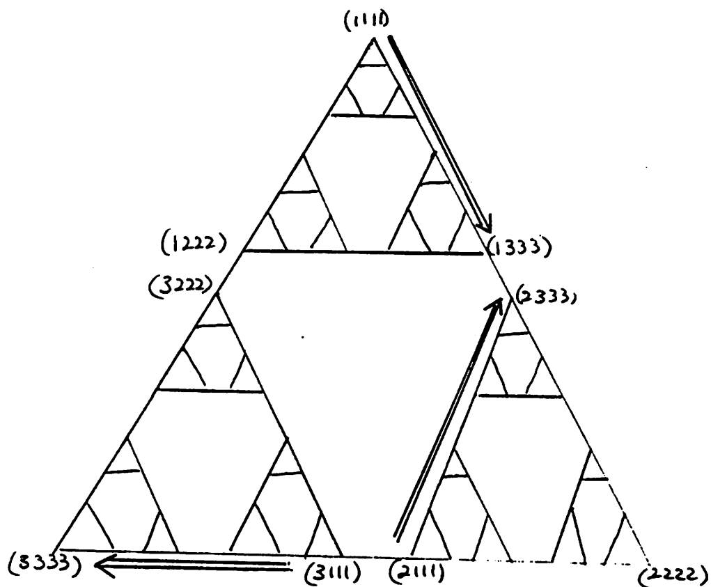
Figure 48: State Transition Graph for Four-Disk Tower of Hanoi Puzzle
