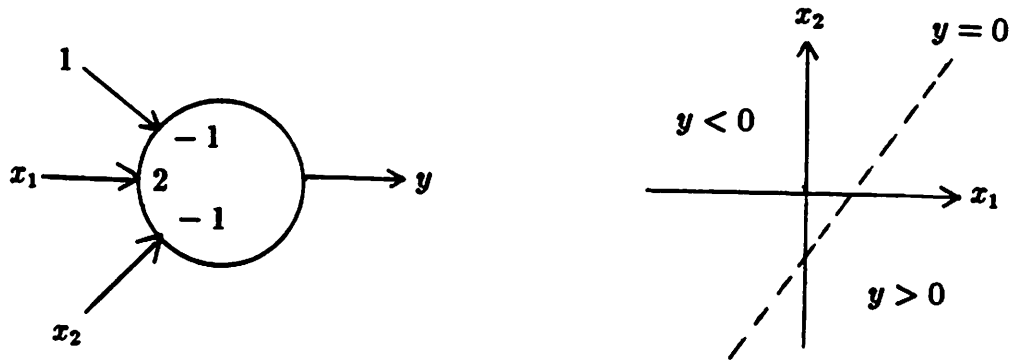
Figure 2: Discrimination of a Linear Threshold Unit
