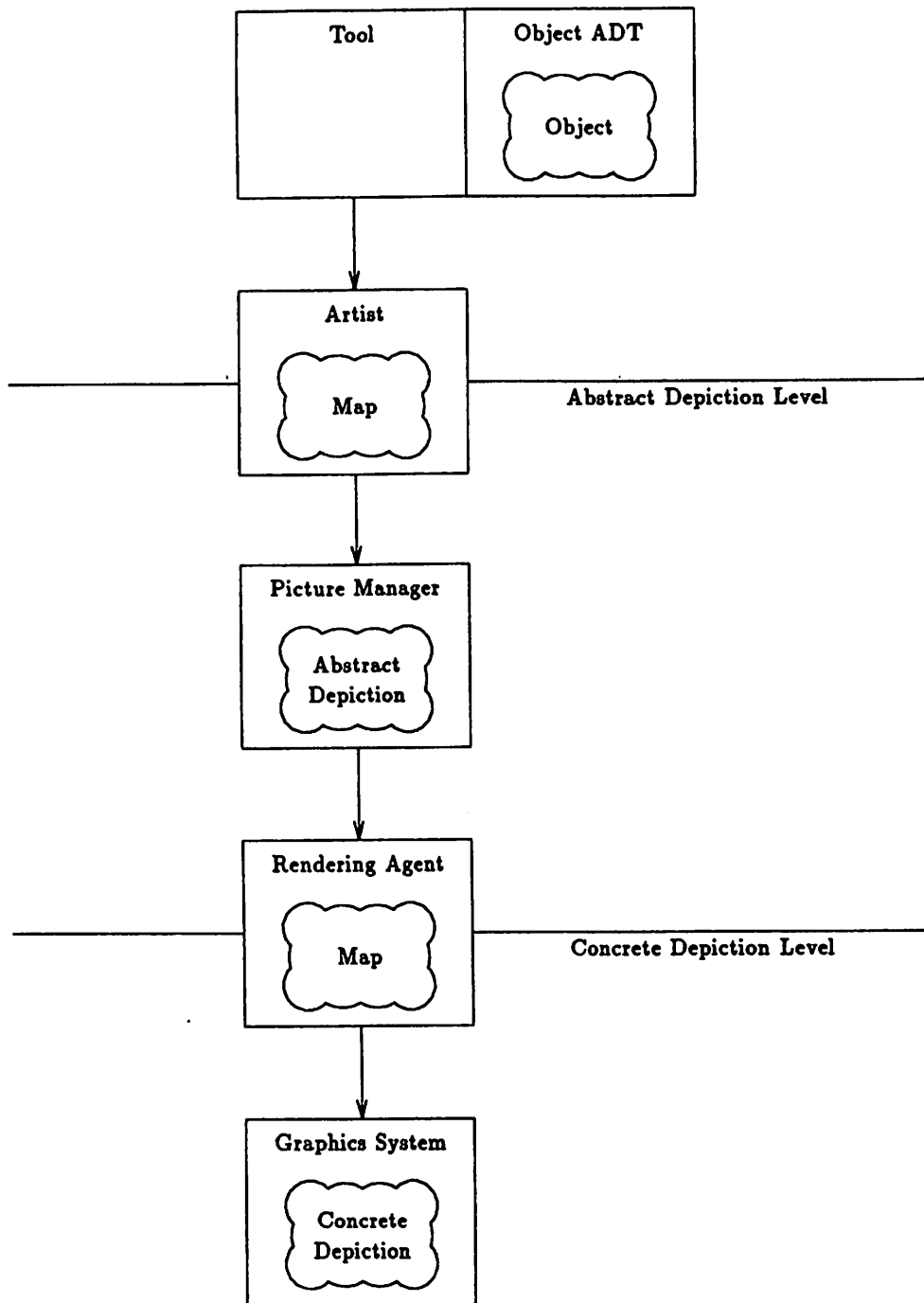
Figure 4: The most difficult part of interactive graphics programming is maintaining the association between application objects and their depictions. When a structured intermediate representation (an abstract depiction ) is interposed between application objects and their depictions, this task can be considerably simplified. The system can maintain the relationship between the abstract and concrete depictions, and associate input events with particular components of the abstract depiction. The artist that created that particular component can then be notified; it need only maintain the relationship between high-level graphical objects and the application objects they depict.
