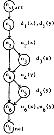
Figure 2: Module M_2 and its control flow graph G(M_2) .
