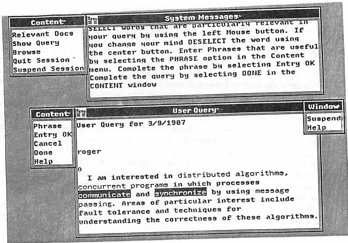
Figure 1: Selecting important words and phrases in I 3 R.
