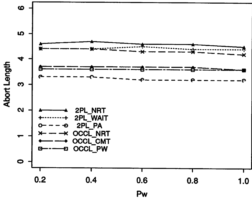
Fig.7: Data contention, MPL = 8, x = 6, a = 5
