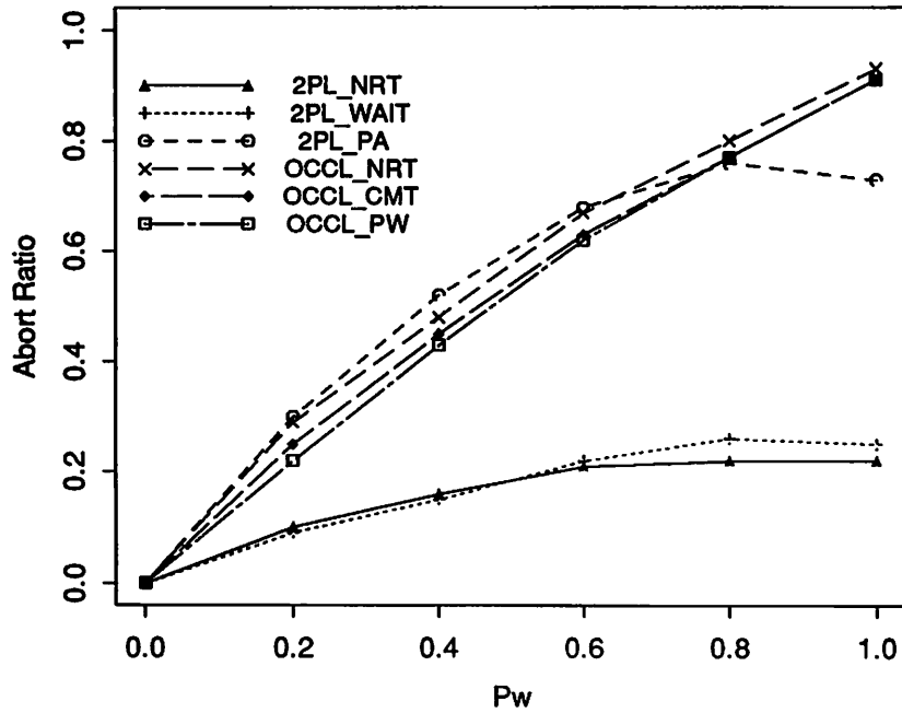
Fig.6: Data contention, MPL = 8, x = 6, a = 5
