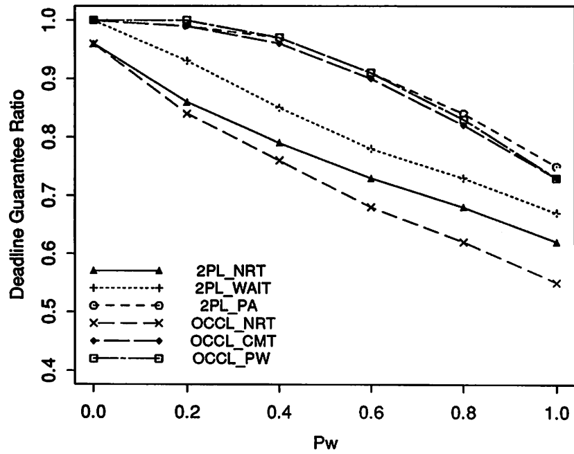
Fig.2: Data contention, MPL = 8, x = 6, a = 5
