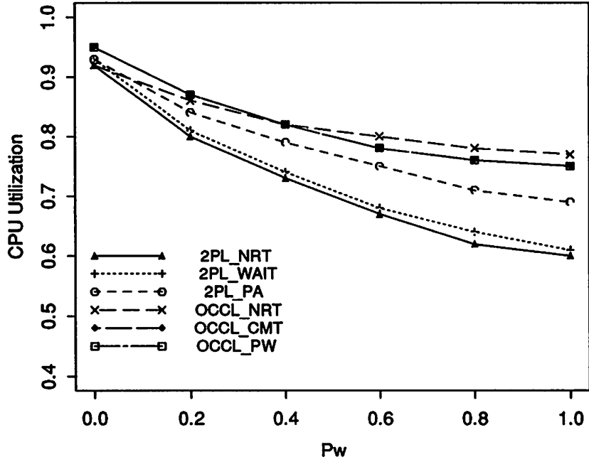
Fig.9: Data contention, MPL = 8, x = 6, a = 5
