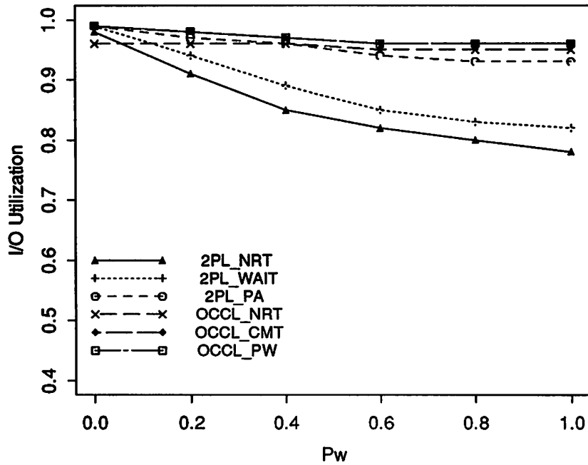
Fig.10: Data contention, MPL = 8, x = 6, a = 5
