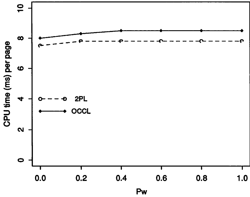
Fig.1: Concurrency control overhead
