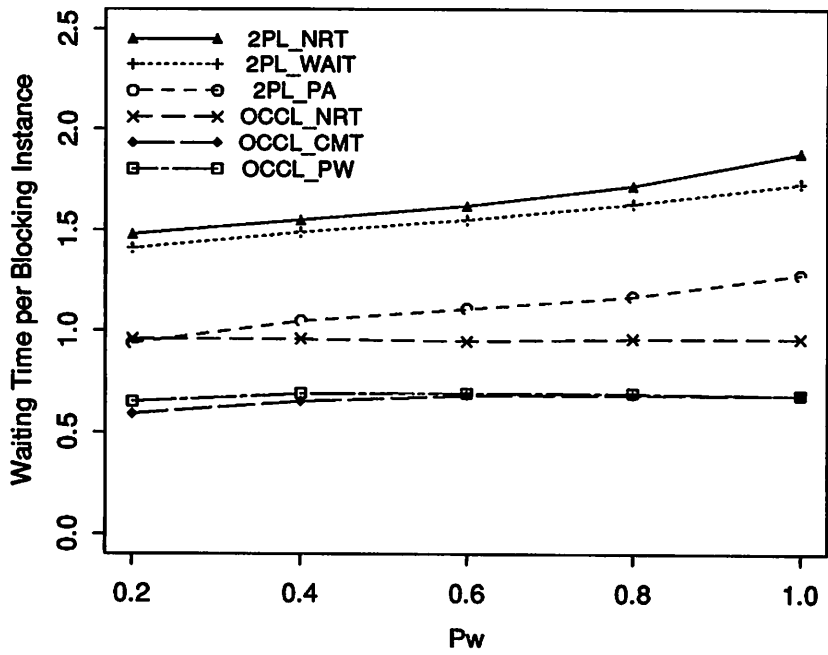
Fig.3: Data contention, MPL = 8, x = 6, a = 5
