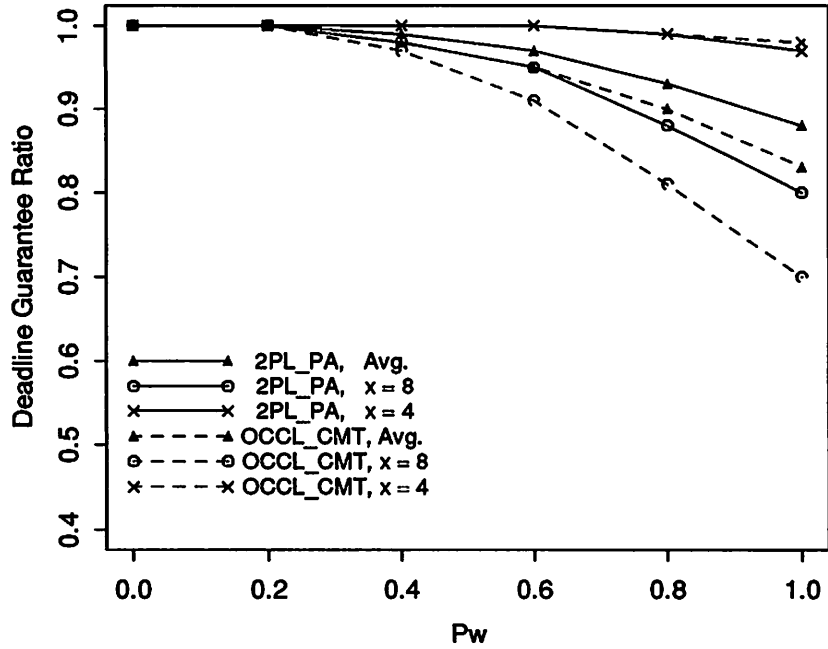
Fig.15: Mixed transactions, MPL = 8, x = [4,8] , a = 5
