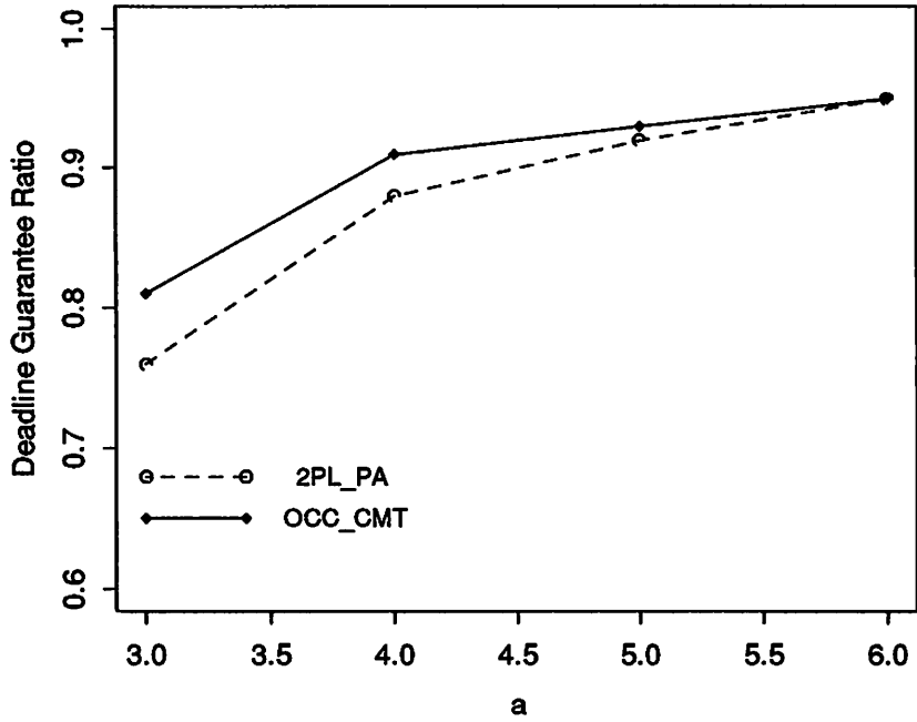
Fig.13: Deadline distribution, MPL = 4, x = 6, Pw = 0.2
