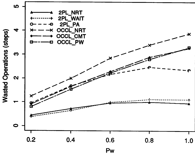
Fig.8: Data contention, MPL = 8, x = 6, a = 5
