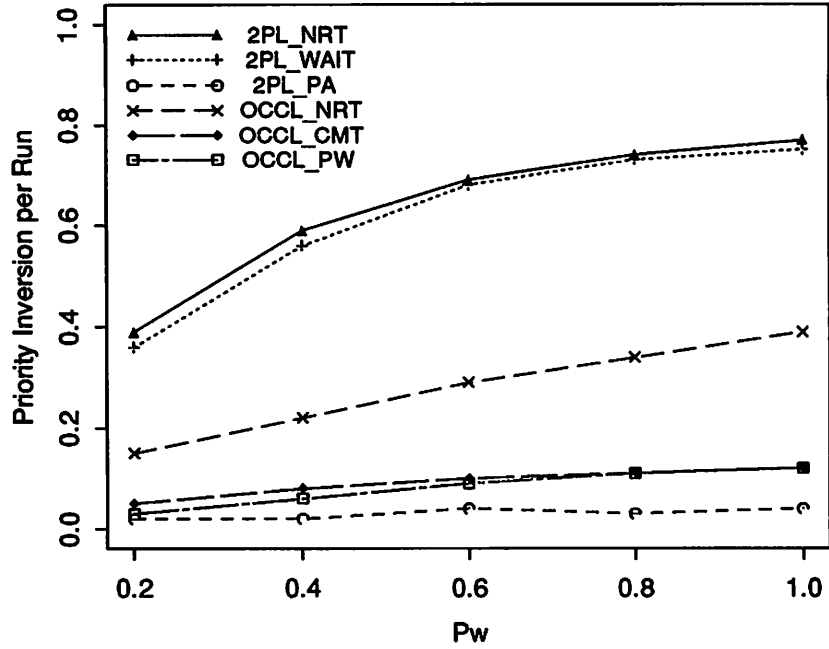
Fig.5: Data contention, MPL = 8, x = 6, a = 5
