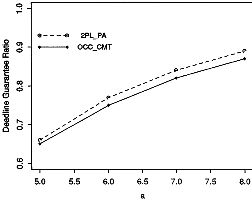
Fig.14: Deadline distribution, MPL = 4, x = 6, Pw = 0.8
