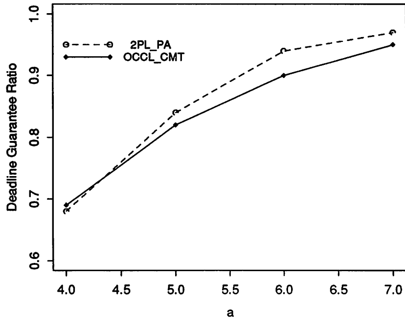
Fig.12: Deadline distribution, MPL = 8, x = 6, Pw = 0.8
