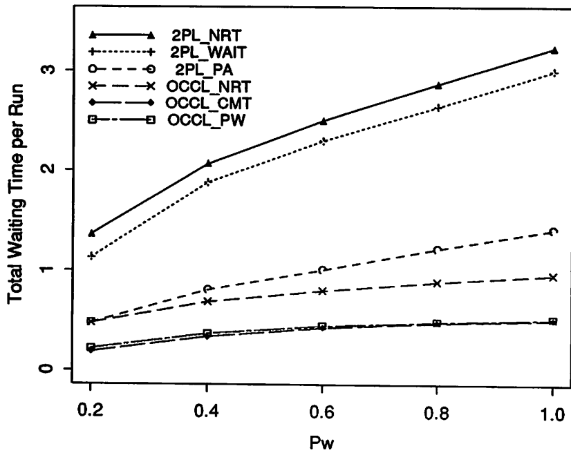
Fig.4: Data contention, MPL= 8, x = 6, a = 5
