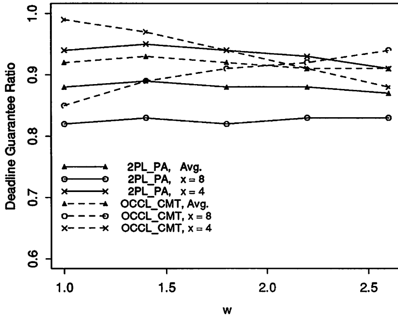
Fig.16: Mixed transactions, MPL = 8, x = [4,8] , P_w = 0.2 , a = 2
