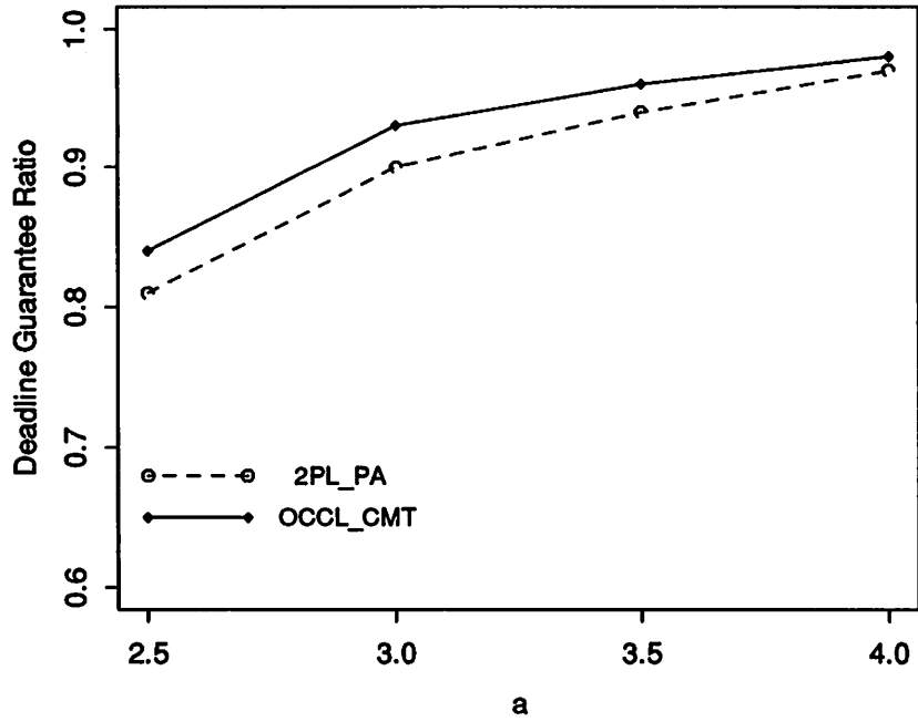
Fig.11: Deadline distribution, MPL = 8, x = 6, Pw = 0.2
