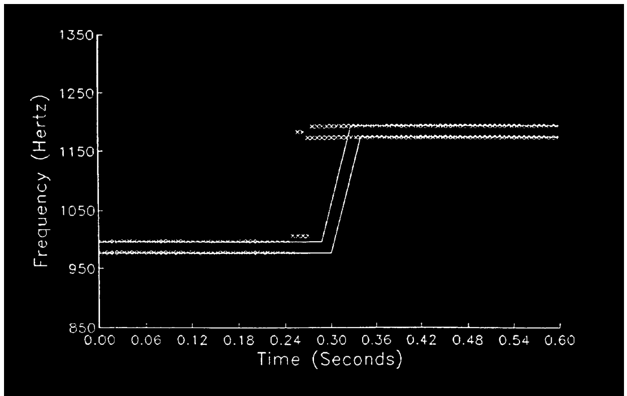
Figure 25: A signal-processing output for a motor sound . The solid lines represent the actual frequency tracks while the \times 's represent the STFT output data. Time-resolution distortion causes the motor speed-change interval not to be tracked.
