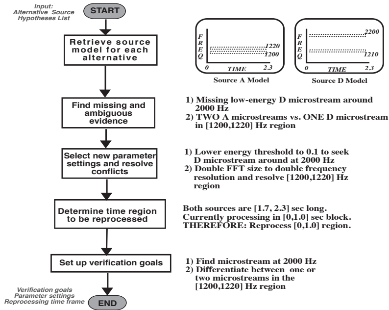
Figure 14: A flowchart for the IPUS differential diagnosis KS and its execution in the testbed scenario.
