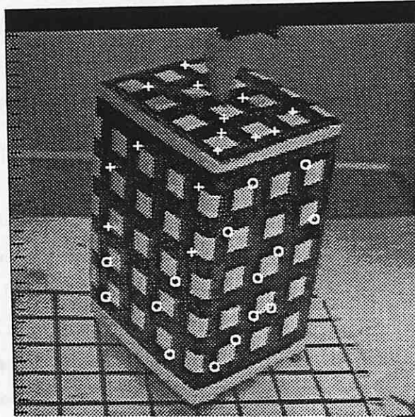
Figure 2: Box Image. The points marked by crosses were used to compute the 3D pose for each frame. Using these poses, the 3D location of the numbered points marked by circles is computed.
