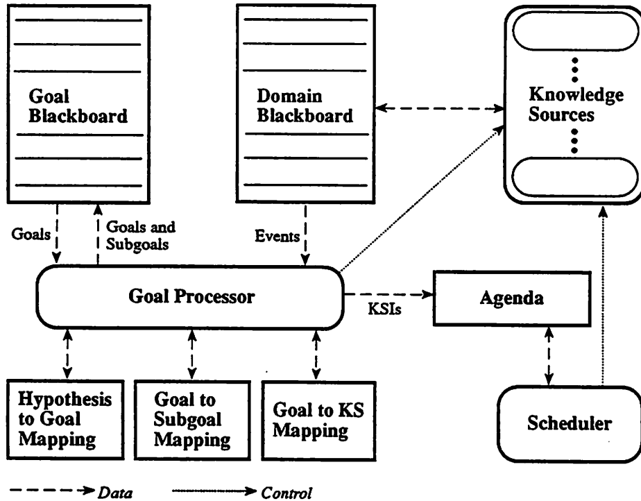
Figure 8: The goal-directed blackboard architecture. Compared to the agenda-based architecture of HSII (Figure 1), the goal-directed architecture adds the goal blackboard and the goal processor replaces the blackboard monitor. The goal processor uses the hypothesis-to-goal , goal-to-subgoal , and goal-to-KS mappings to post goals/subgoals and trigger KSs.
