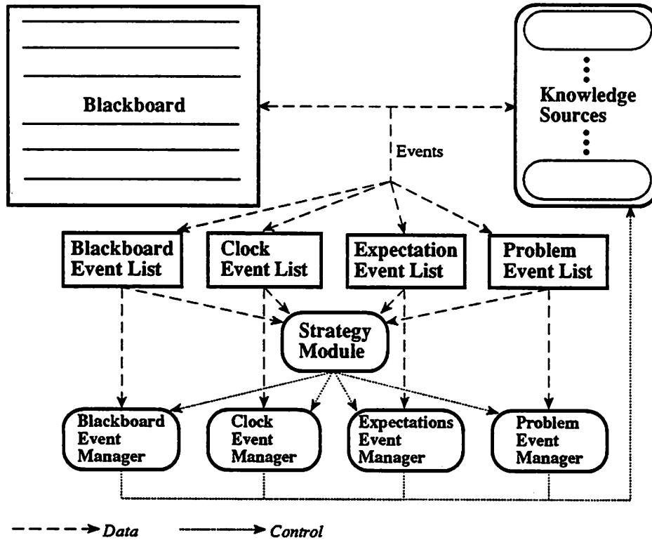
Figure 4: The HASP/SIAP blackboard architecture.
