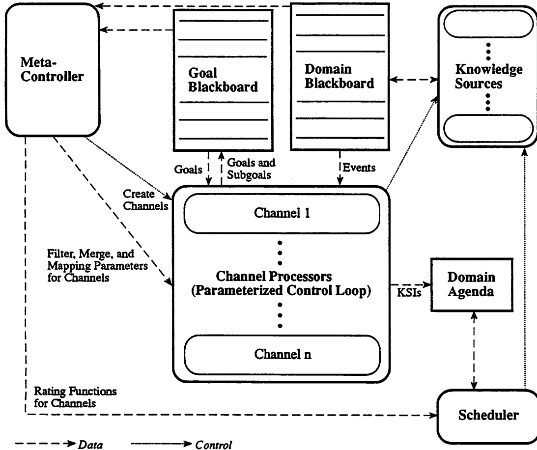
Figure 11: The channelized, parameterized blackboard architecture. Compared to the goal-directed blackboard architecture (Figure 8), the goal-directed architecture adds the meta-controller (see Figure 12) and the channel processors replace the goal processor. The channel processors execute the parameterized control loop (Figure 13) that is an extension of the control loop used in the goal-directed blackboard architecture. In addition to the hypothesis-to-goal , goal-to-subgoal , and goal-to-KS mappings done by the goal processor, the channel processors do hypothesis filtering , goal filtering , goal merging, and KSI merging. The meta-controller is responsible for creating channels; setting the filtering, merging, and mapping parameters for the channels; and determining the rating functions for KSIs associated with each channel.
