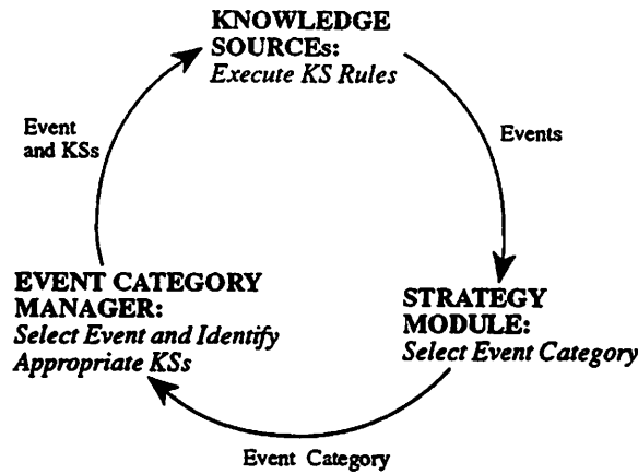
Figure 5: The basic control loop for HASP.
