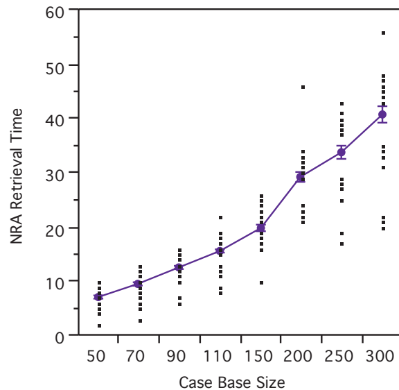
Figure 2: Negotiated Retrieval Time versus Casebase Size
