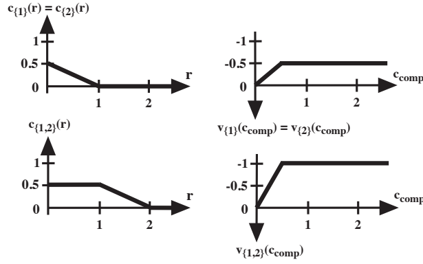
Figure 3: Performance profiles and value functions of the counterexample.
