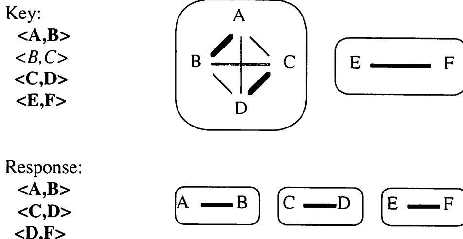
Figure 6.5 Complete graphs representing phrases \{A, B\} , \{C, D\} and \{E, F\}
