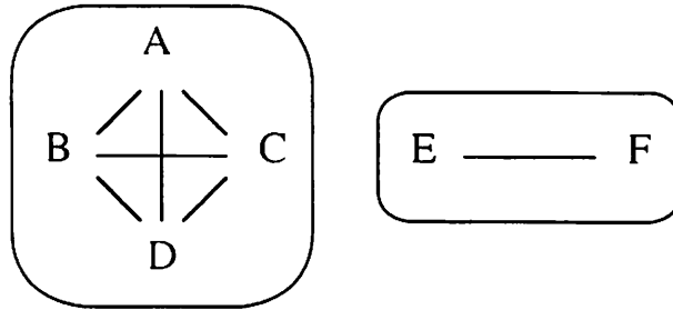
Figure 6.3 Complete graphs representing phrases \{A, B, C, D\} and \{E, F\}
