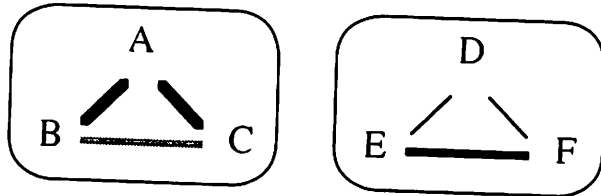
Figure 6.4 Complete graphs representing phrases {A, B, C} and {D, E, F}
