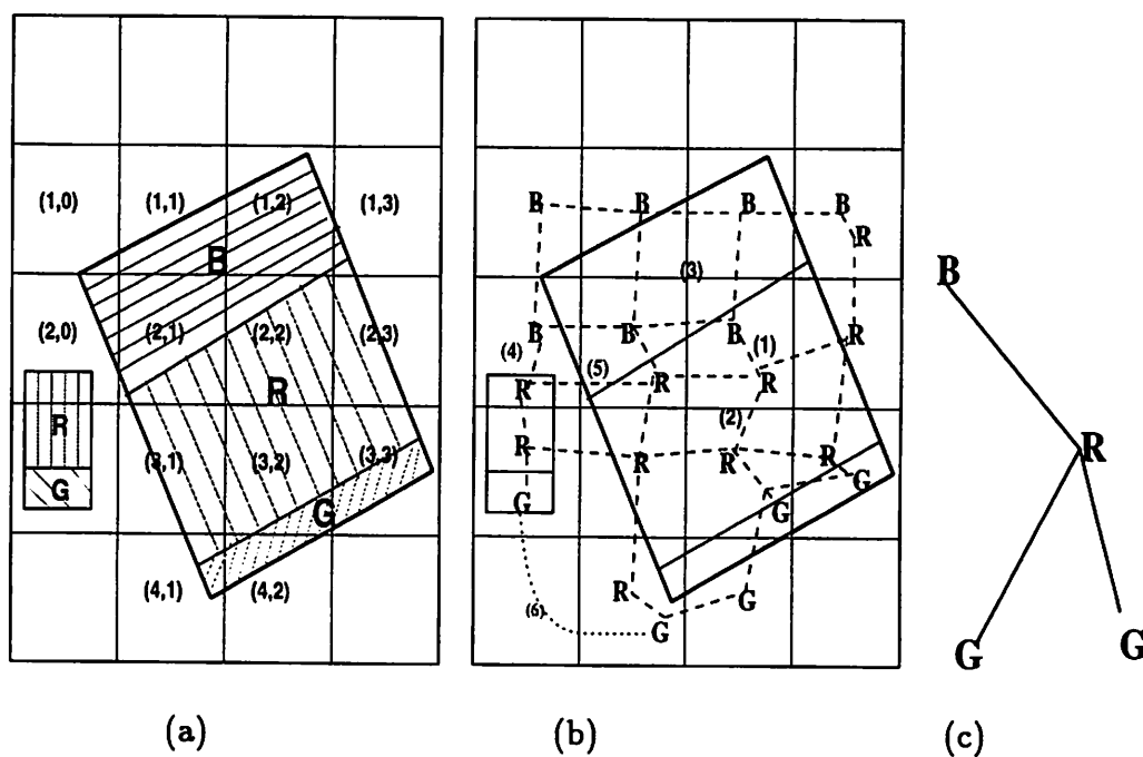
Figure 7: Example of CNG construction (a) Synthetic image divided into cells (b) Cells marked with nodes (peaks) contained in them. The edges between the nodes are shown in broken lines (c) Final CNG after merging
