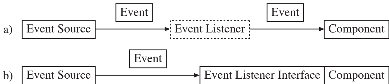
Figure 1: Event propagation model for (a) “dynamic” links created with beanbox and (b) “static” links specified in the component source code.
