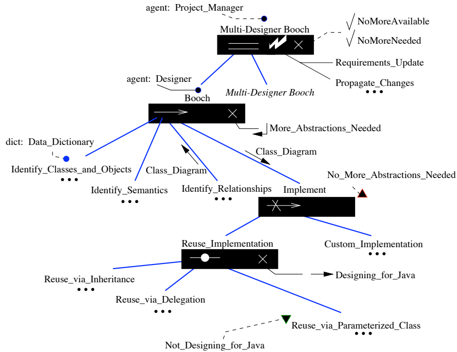
Fig. 1. A Multi-User Booch Process (BOOD) in Little-JIL
