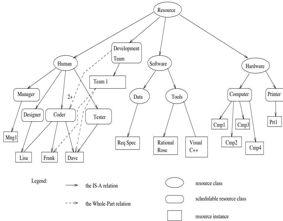
Fig. 3. IS-A and Whole-Part relations
