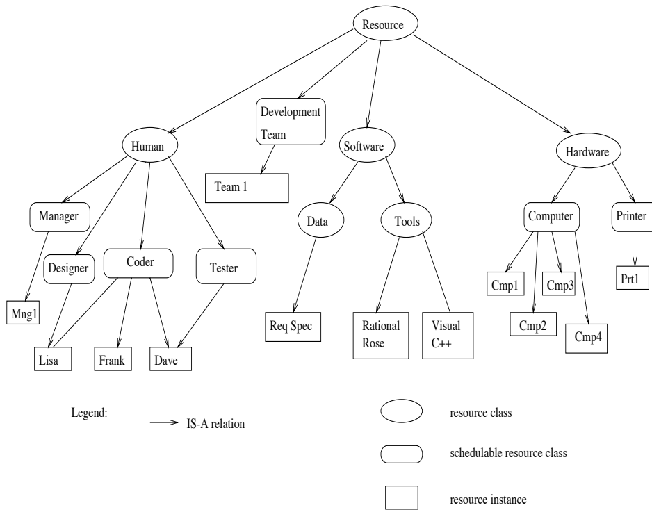
Fig. 1. IS-A hierarchy of an example environment
