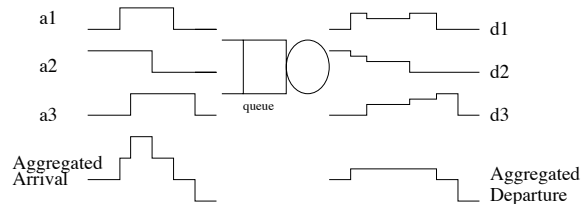
Figure 16: Example of flow aggregation
