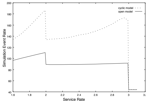
Figure 13: Simulation event rates
