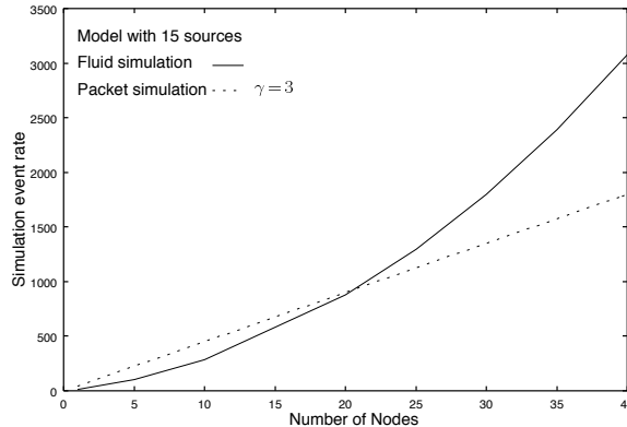
Figure 7: Simulation event rate of a tandem system
