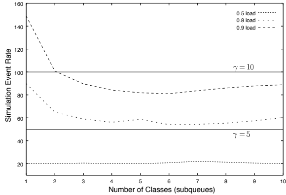
Figure 19: Simulation event rate vs. the number of classes in a WFQ node
