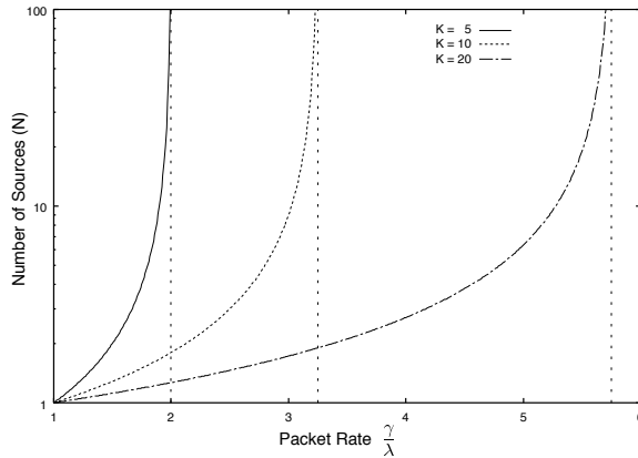
Figure 9: Boundary condition for efficiency and regions between fluid and packet simulation
