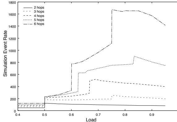
Figure 14: Simulation Event rate for a 6-node cyclic queue
