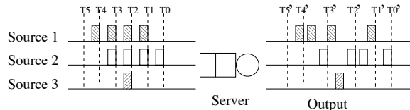
Figure 3: Dynamics of a FIFO packet multiplexer
