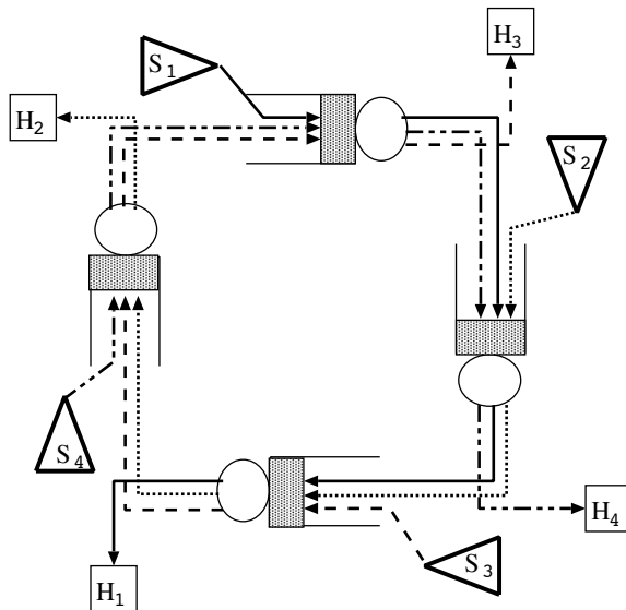
Figure 10: A feedback queueing model
