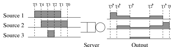
Figure 4: Dynamics of a FIFO fluid multiplexer
