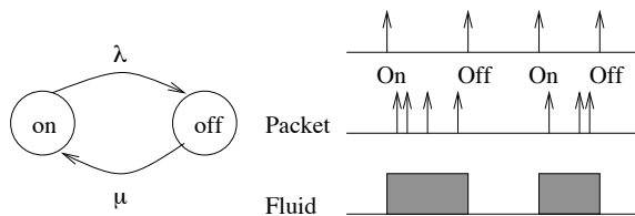
Figure 2: The on-off fluid source and packet source
