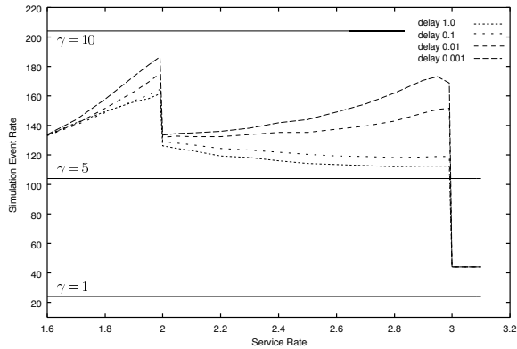
Figure 11: Simulation event rate for the feedback queueing model
