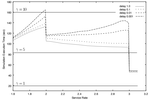
Figure 15: Measured simulation execution time vs service rate
