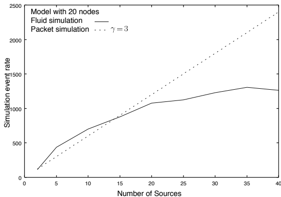
Figure 8: Simulation event rate of a tandem system
