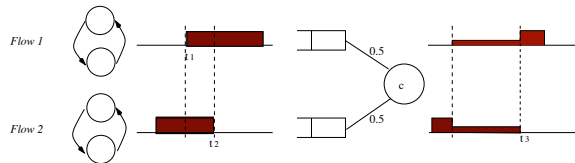
Figure 18: A two queue weighted fair queueing system
