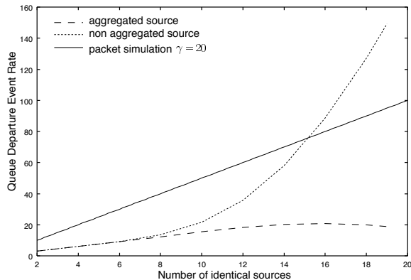
Figure 17: Event rate of flow aggregation and no aggregation
