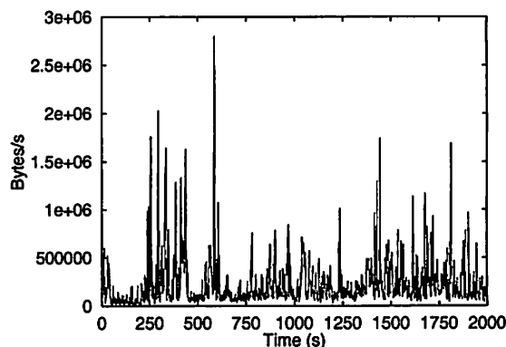
Figure 4: Bursty nature of the NFS trace workload.
