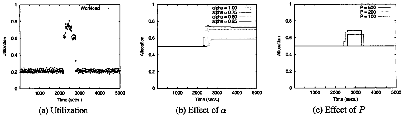
Figure 8: Effect of various tunable parameters on the granularity of bandwidth allocations.
