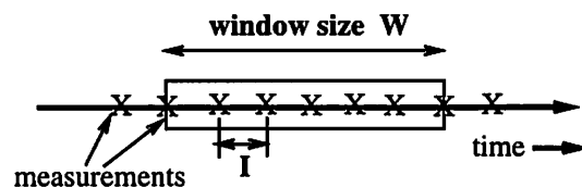
Figure 2: A Moving Histogram
