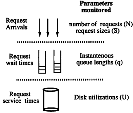
Figure 3: Parameters tracked by the monitoring module
