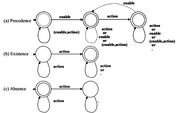
Figure 2. The Other Property Patterns' FSA Templates
