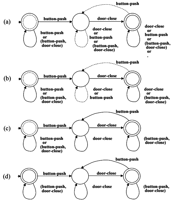
Figure 4. An Example of the PROPEL Process
