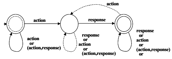
Figure 1. Response FSA Template
