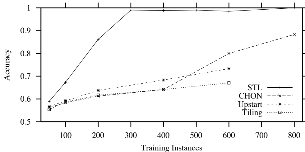
Figure 8. Two-or-more clumps accuracy for several algorithms.
