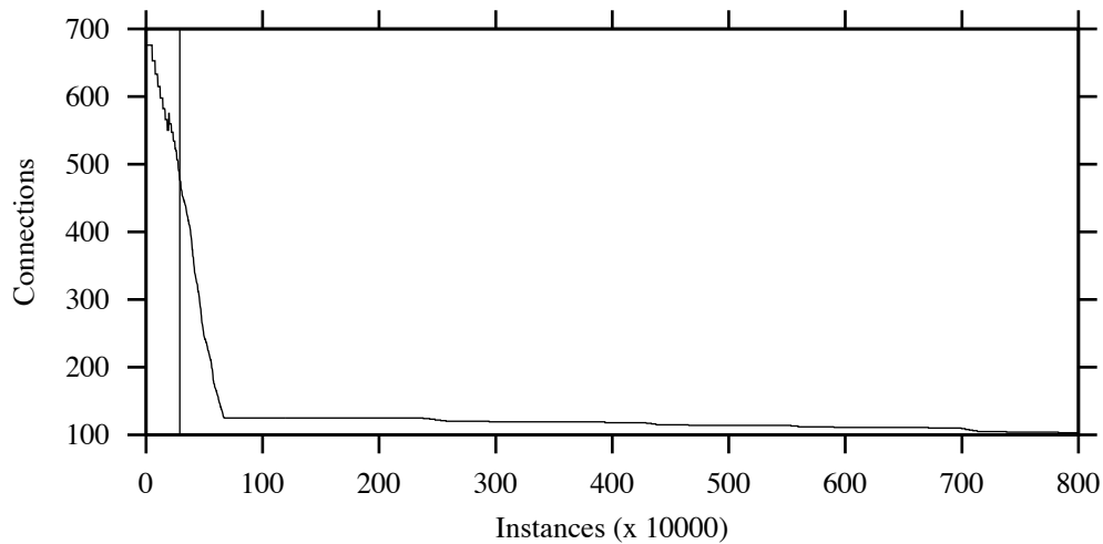
Figure 7. STL total connections while training two-or-more-clumps.
