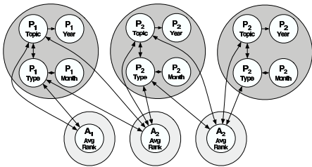
Figure 2. Example PRM inference graph.
