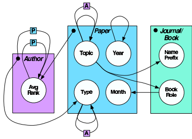
Figure 4. Cora machine-learning papers RDN.
