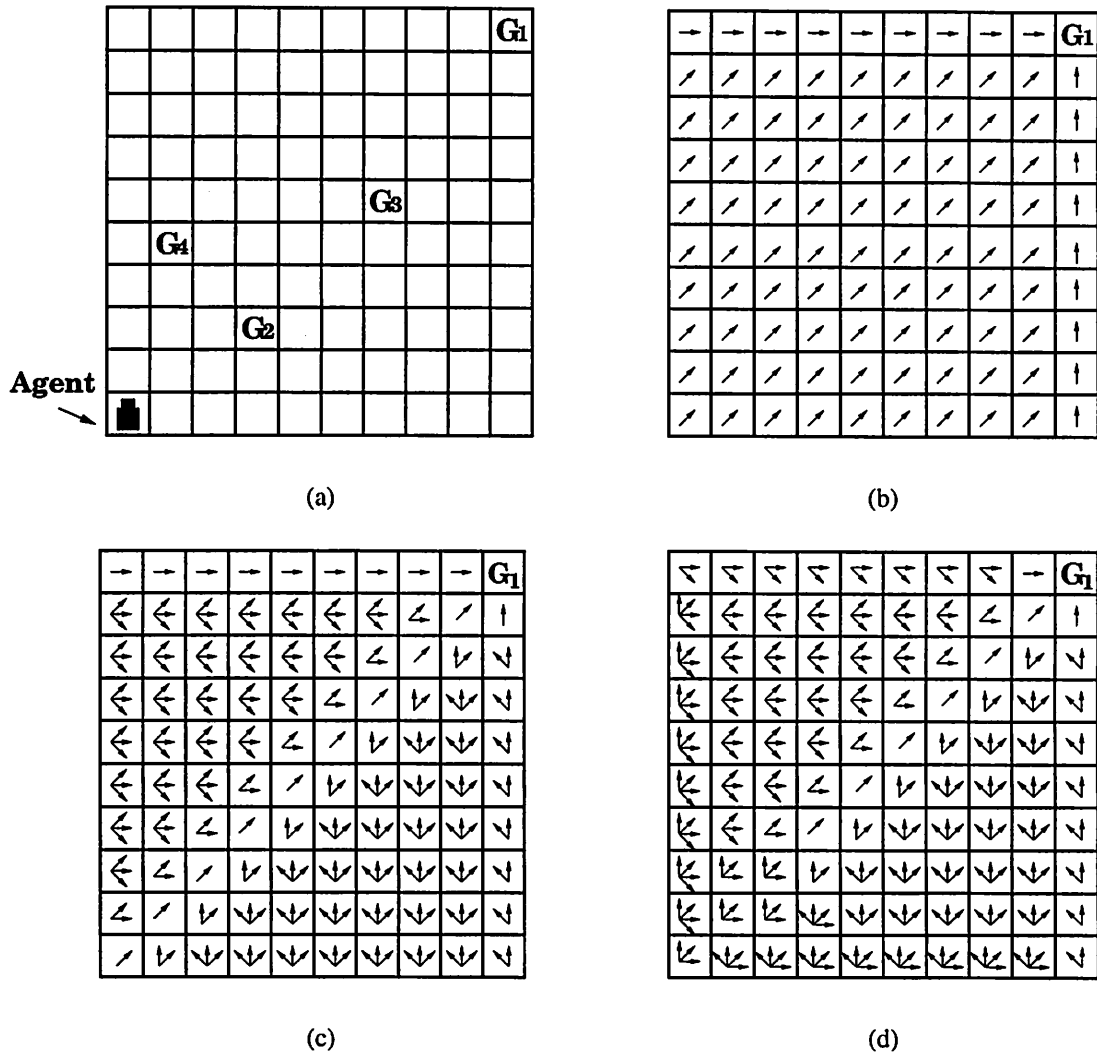
Figure 2: (a) A 10 × 10 grid world where an agent is to visit a set of prioritized subgoal locations; (b) The optimal policy associated with the subgoal G_1 ; (c) The \epsilon -ascending policy for \epsilon = 0.95 ; (d) The \epsilon -ascending policy for \epsilon = 0.90 .
