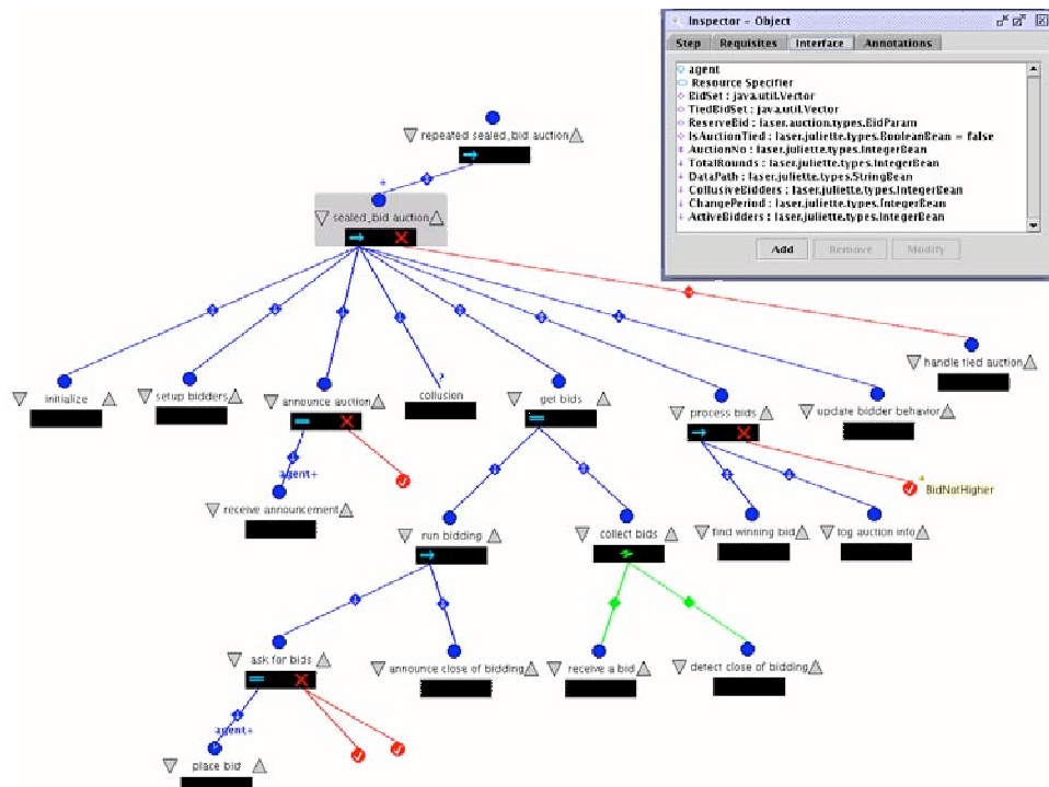
Fig. 4. A repeated sealed-bid auction process
