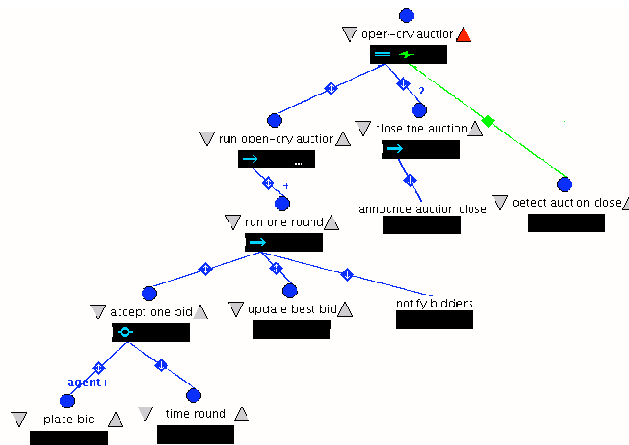
Fig 2. An Open-cry (Ascending bid/English) auction
