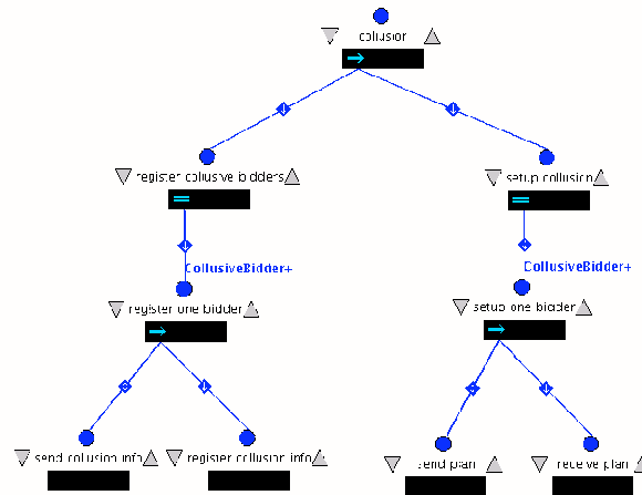
Fig. 5.. A Collusion Process in Sealed-bid Auction
