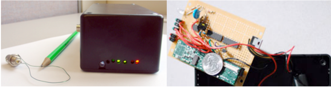
Fig. 1. Our assembled PICCAL credit card emulator
