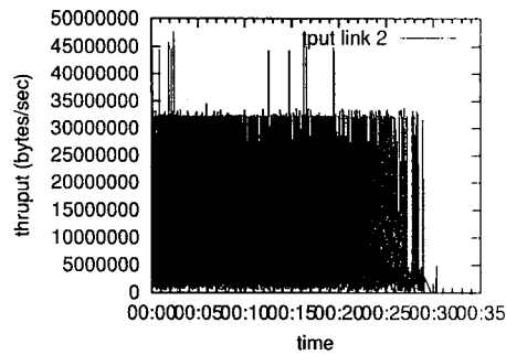
Fig. 12. Throughput on link 2 (average over 10 segments)
