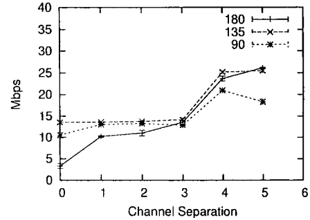
Fig. 3. Throughput results for the routing case with varying antenna separation ( 180^\circ , 135^\circ , 90^\circ )
