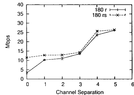
Fig. 7. Throughput results for additional separation in the vertical (180° setup. 'r' routing without vertical separation, 'rs' routing and 4 ft vertical separation)
