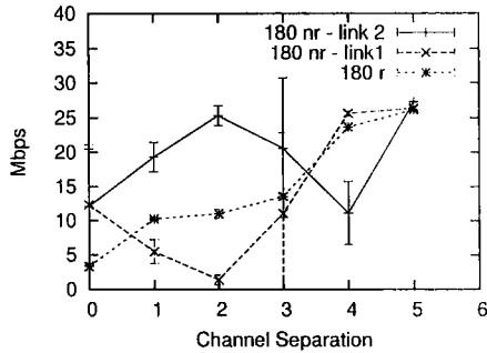
Fig. 2. Throughput results for routing vs. non-routing ( 180^\circ )
