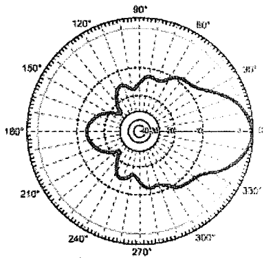
Fig. 5. Antenna pattern
