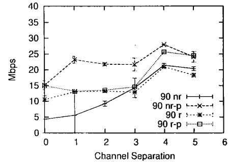
Fig. 6. Throughput results for changed and non-changed polarization on link 2
