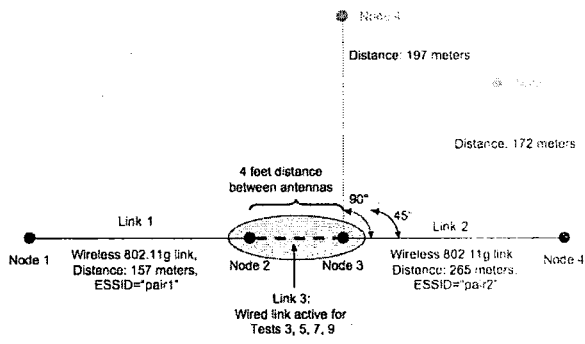
Fig. 1. Measurement setup
