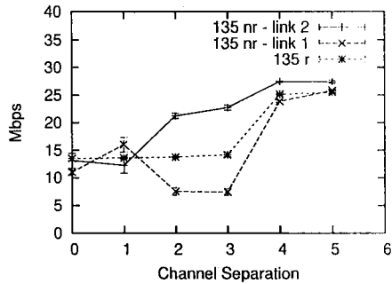
Fig. 4. Throughput results for routing and non-routing in the 135° case
