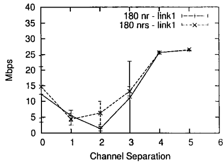
Fig. 8. Throughput results for link 1 with (nrs) and without (nr) additional separation in the vertical ( 180^\circ setup)
