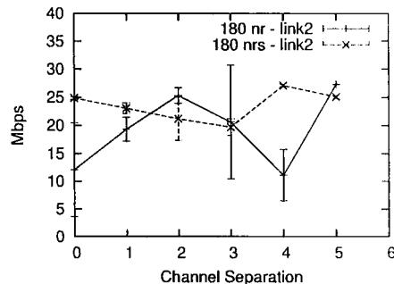
Fig. 9. Throughput results for link 2 with (nrs) and without (nr) additional separation in the vertical ( 180^\circ setup)
