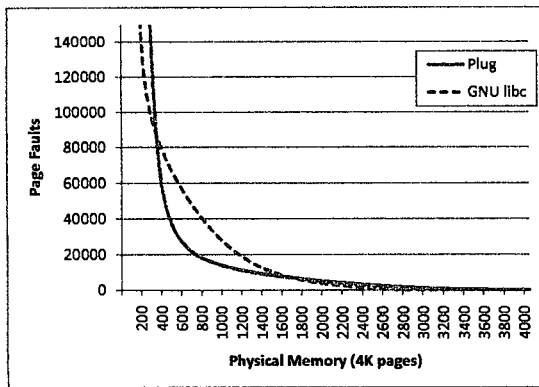
(b) 10% leak rate
