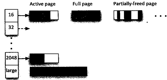
Figure 4. Plug's age-segregated heap (see Section 3.2).
