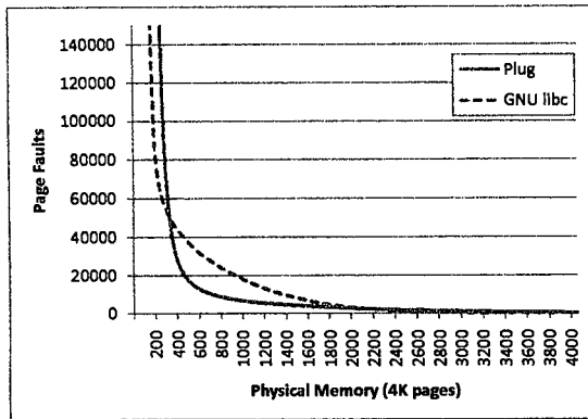
(a) 50% leak rate
