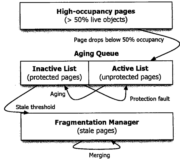
Figure 8. The life cycle of a page in Plug (see Section 4.2.1).
