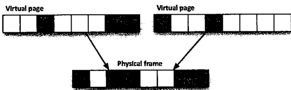
Figure 7. An example pair of pages that share no common live indices. The virtual compactor can merge these pages in physical memory while not actually relocating objects in virtual memory (see Section 4).
