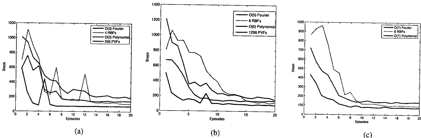
Figure 2: Learning curves for agents using (a) order 3 (b) order 5 and (c) order 7 Fourier Bases, and RBFs and PVFs with corresponding number of basis functions.
