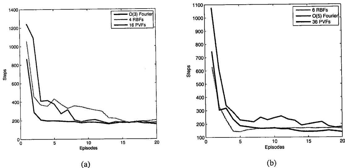
Figure 7: Learning curves for agents using (a) order 3 (b) order 5 Fourier Bases, and RBFs and PVFs with corresponding number of basis functions.
