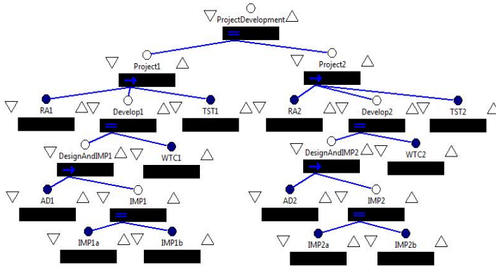
Fig. 1. Project development process described by Little-JIL
