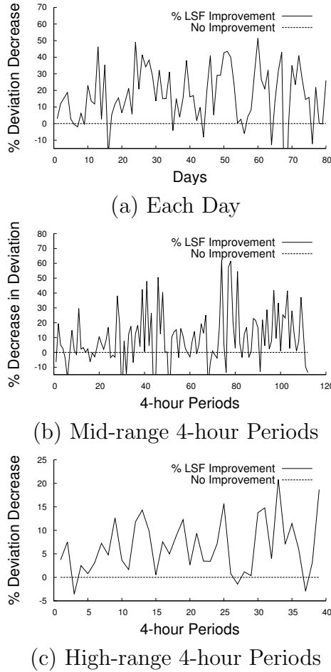
Figure 3.8. LSF decreases the absolute average deviation from the mean power (with no scheduling) on the vast majority of days (91%), as well as over peak 4-hour periods with mid-range and high-range deviations.
