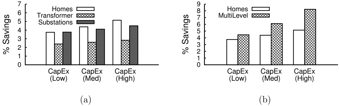
Figure 7.5. Savings from deploying lead-acid battery storage at (a) single level and (b) multiple levels under the long-term contract pricing plan.
